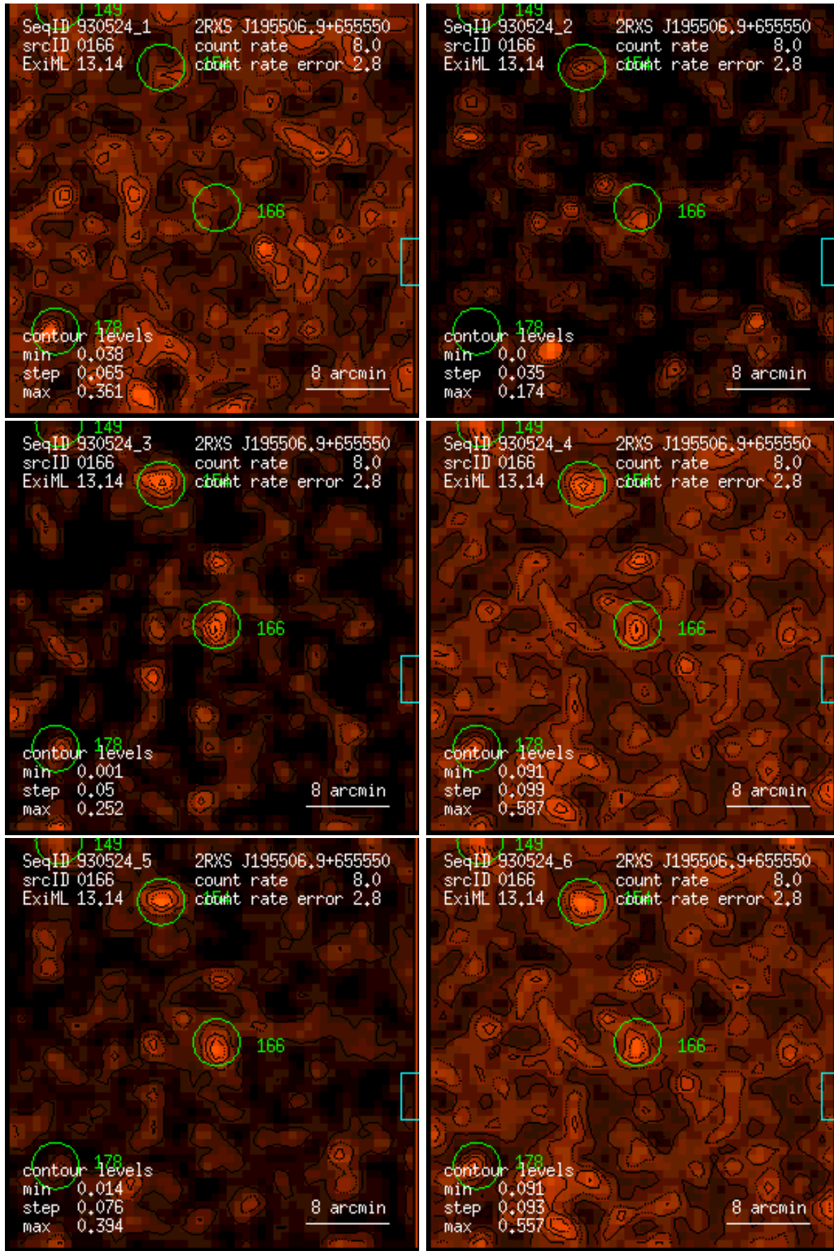
Figure 166: RASS 930524: detection 0166: band rate images, Gaussian filter: (1) PSPC channels 11 – 41, (2) 52 – 90, (3) 91 – 201, (4) 11 – 235, (5) 52 – 201, (6) 11 – 201. Broad band rates in counts/ks. Band rate contour levels in counts/ks/arcmin 2 .
