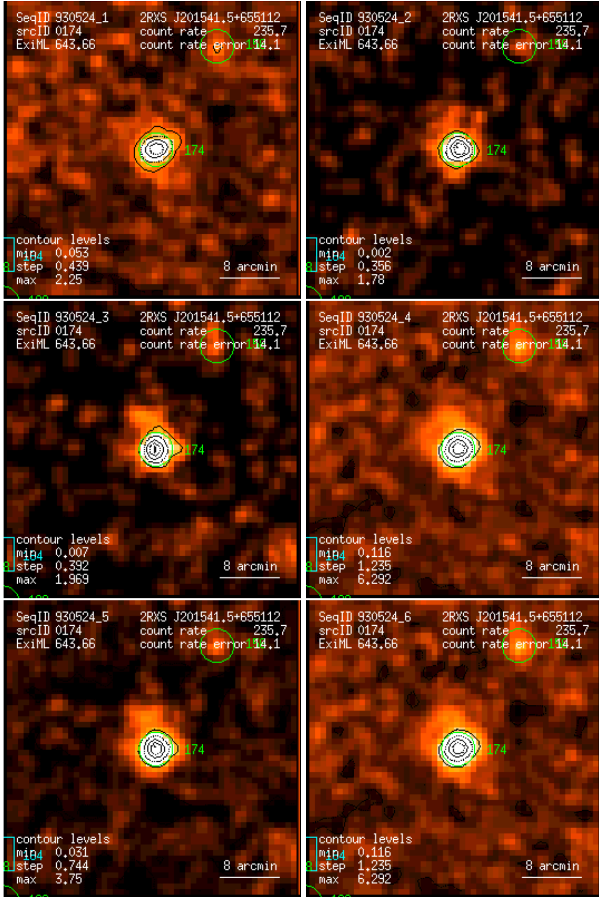
Figure 174: RASS 930524: detection 0174: band rate images, Gaussian filter: (1) PSPC channels 11 – 41, (2) 52 – 90, (3) 91 – 201, (4) 11 – 235, (5) 52 – 201, (6) 11 – 201. Broad band rates in counts/ks. Band rate contour levels in counts/ks/arcmin 2 .
