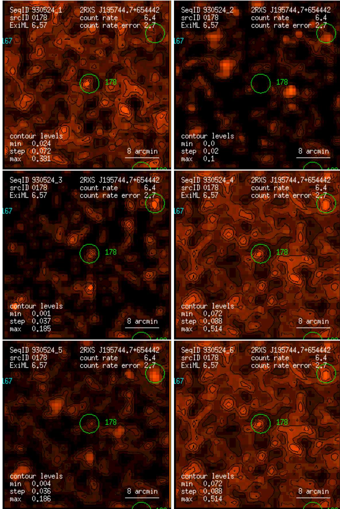
Figure 178: RASS 930524: detection 0178: band rate images, Gaussian filter: (1) PSPC channels 11 – 41, (2) 52 – 90, (3) 91 – 201, (4) 11 – 235, (5) 52 – 201, (6) 11 – 201. Broad band rates in counts/ks. Band rate contour levels in counts/ks/arcmin 2 .
