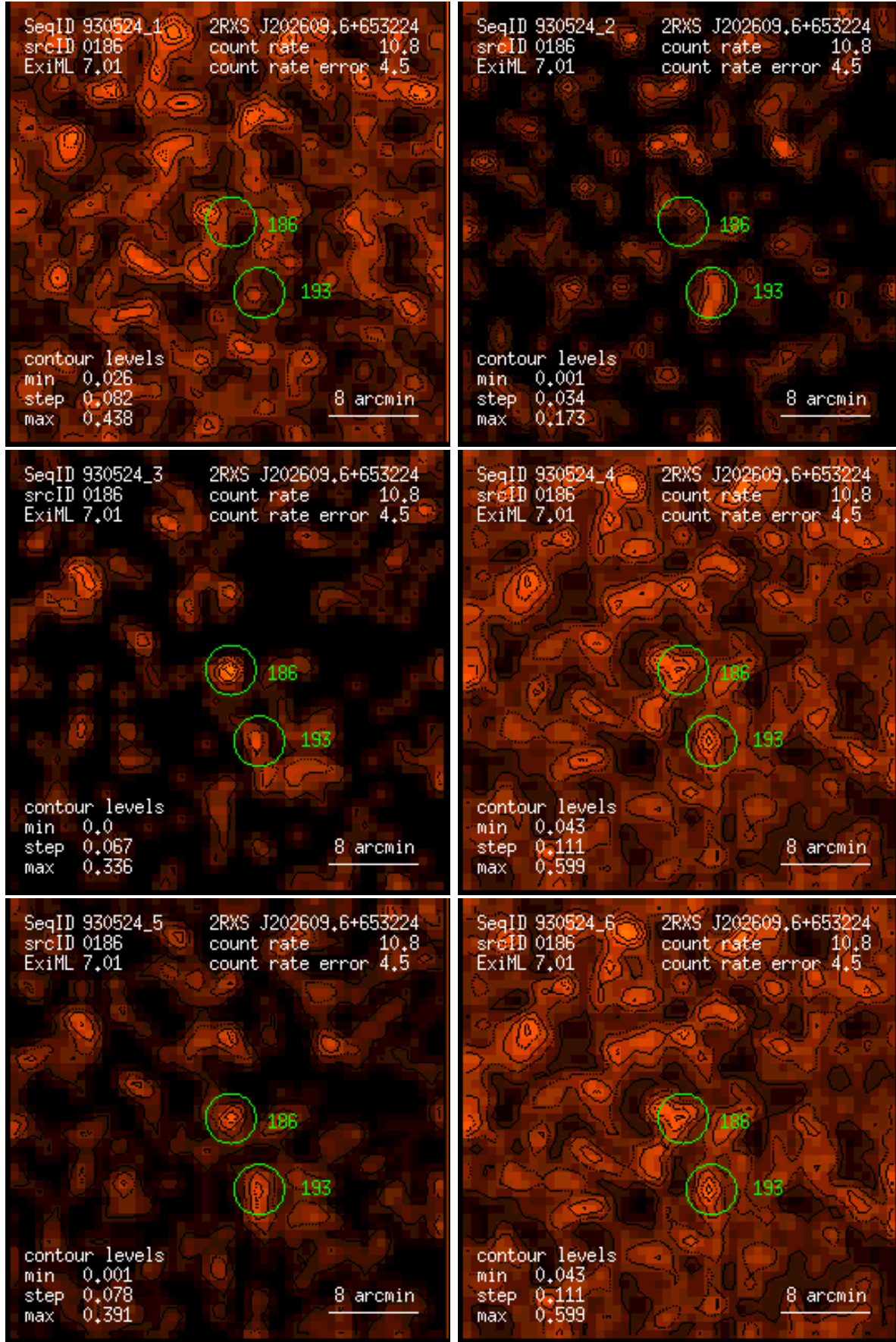
Figure 186: RASS 930524: detection 0186: band rate images, Gaussian filter: (1) PSPC channels 11 – 41, (2) 52 – 90, (3) 91 – 201, (4) 11 – 235, (5) 52 – 201, (6) 11 – 201. Broad band rates in counts/ks. Band rate contour levels in counts/ks/arcmin 2 .
