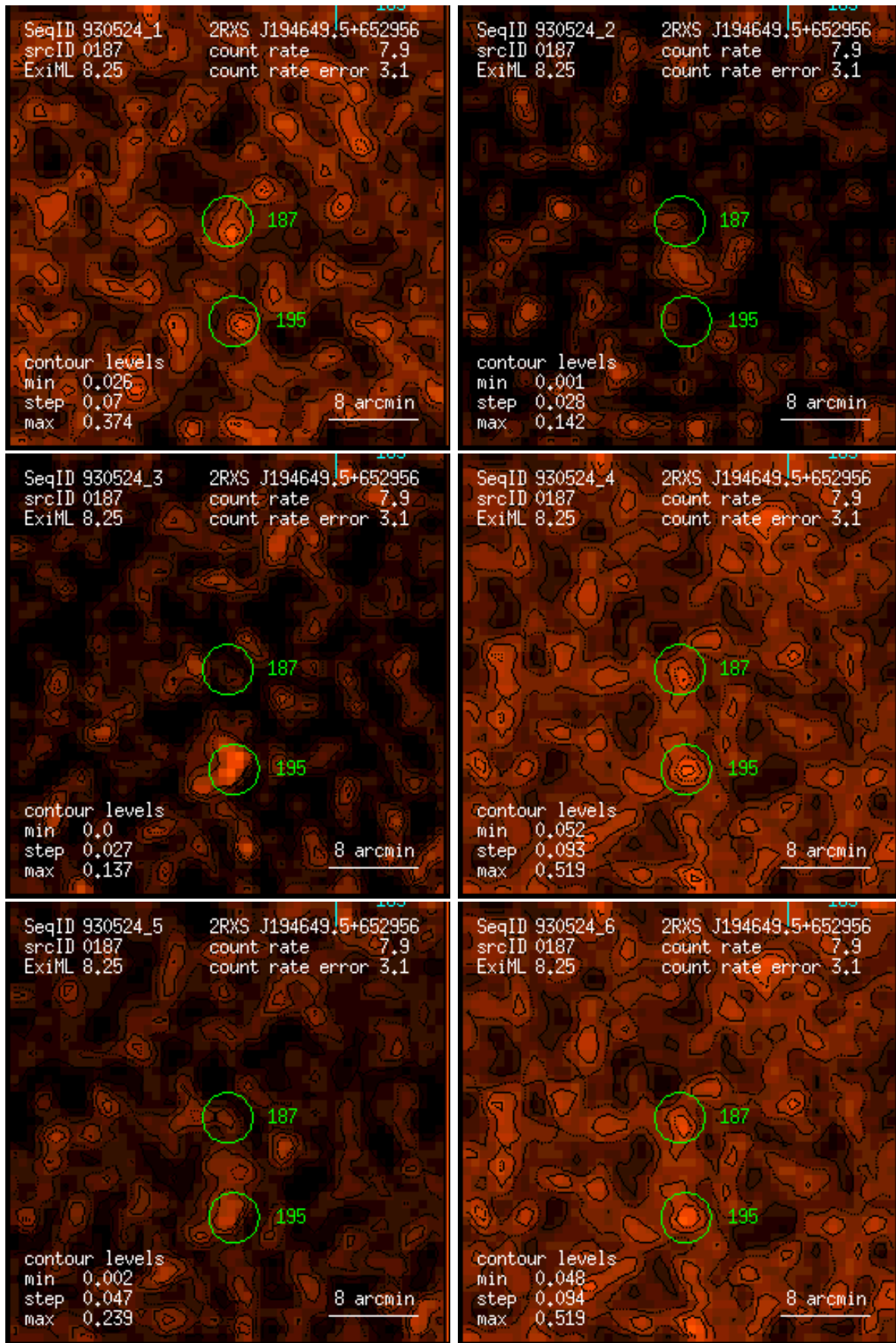
Figure 187: RASS 930524: detection 0187: band rate images, Gaussian filter: (1) PSPC channels 11 – 41, (2) 52 – 90, (3) 91 – 201, (4) 11 – 235, (5) 52 – 201, (6) 11 – 201. Broad band rates in counts/ks. Band rate contour levels in counts/ks/arcmin 2 .
