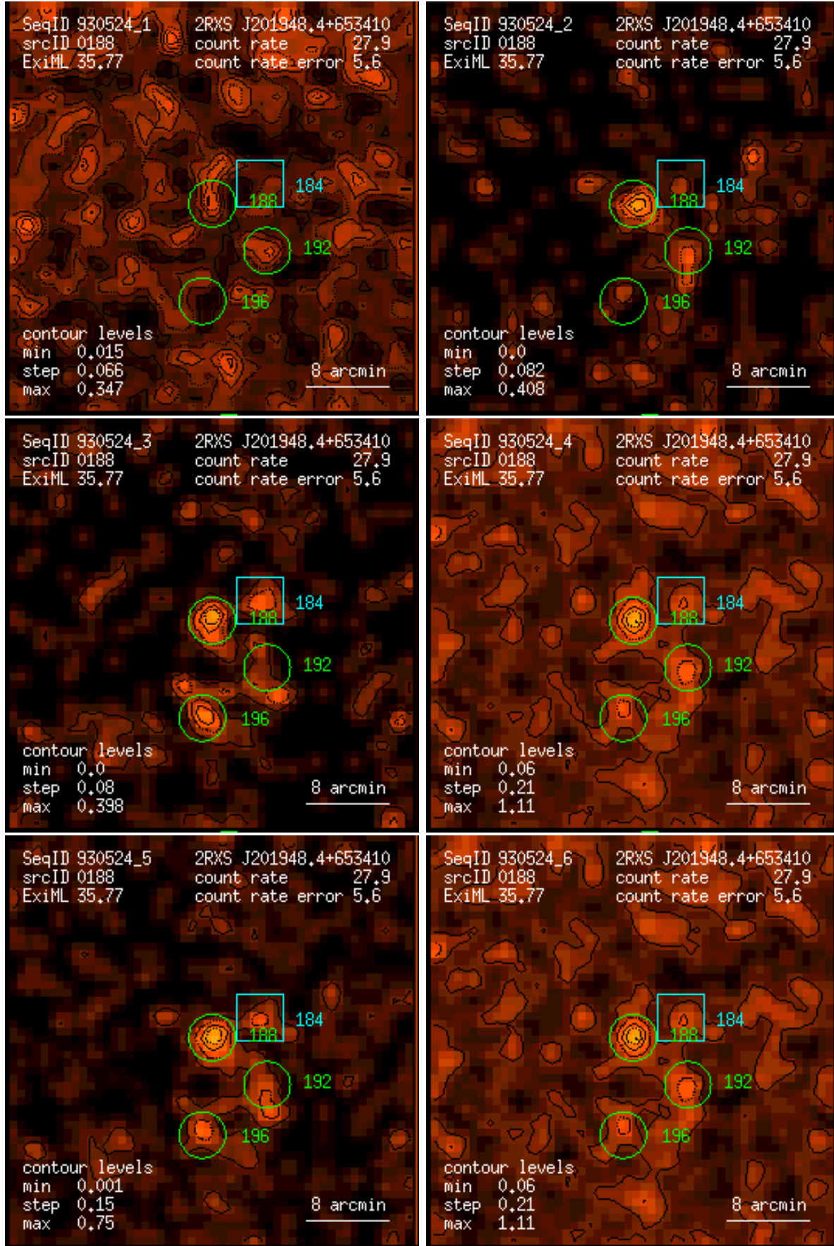
Figure 188: RASS 930524: detection 0188: band rate images, Gaussian filter: (1) PSPC channels 11 – 41, (2) 52 – 90, (3) 91 – 201, (4) 11 – 235, (5) 52 – 201, (6) 11 – 201. Broad band rates in counts/ks. Band rate contour levels in counts/ks/arcmin 2 .
