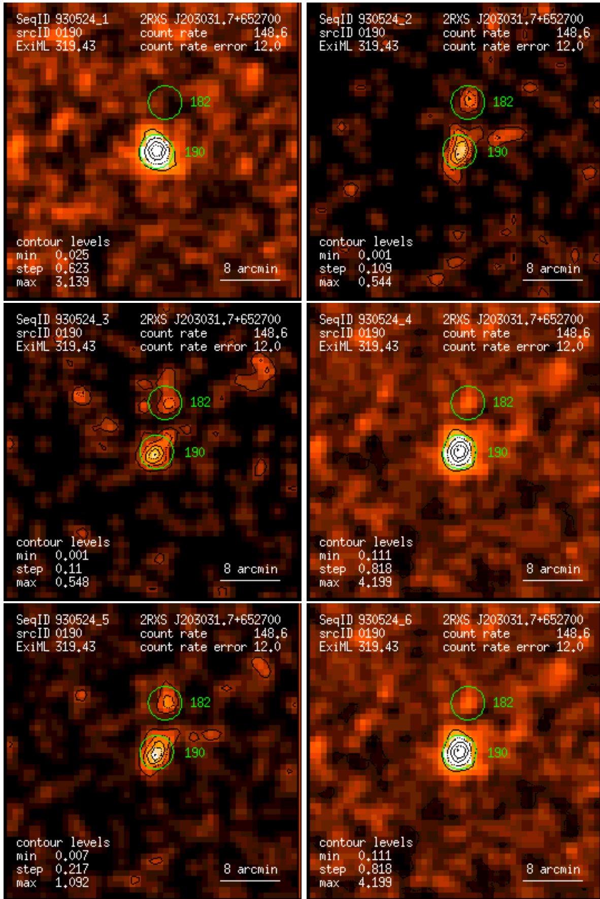
Figure 190: RASS 930524: detection 0190: band rate images, Gaussian filter: (1) PSPC channels 11 – 41, (2) 52 – 90, (3) 91 – 201, (4) 11 – 235, (5) 52 – 201, (6) 11 – 201. Broad band rates in counts/ks. Band rate contour levels in counts/ks/arcmin 2 .
