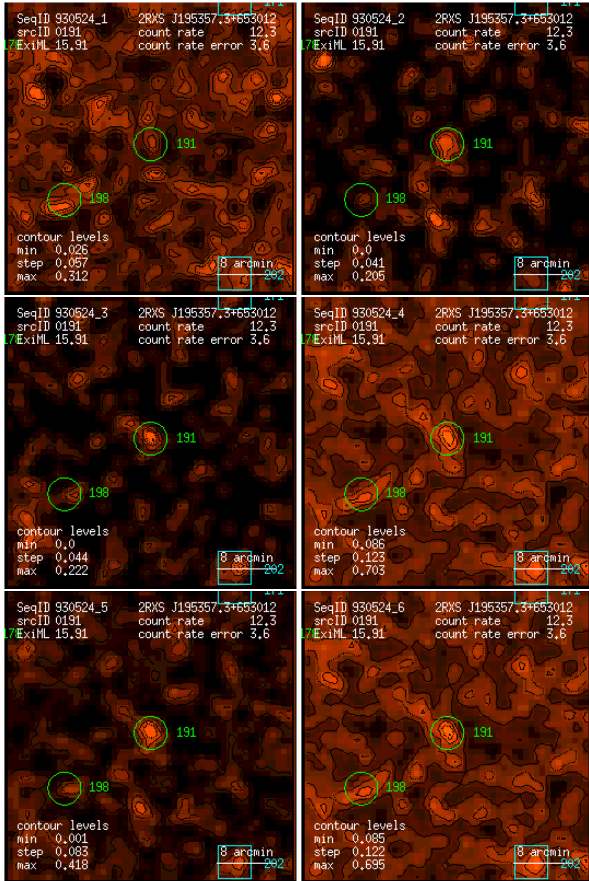
Figure 191: RASS 930524: detection 0191: band rate images, Gaussian filter: (1) PSPC channels 11 – 41, (2) 52 – 90, (3) 91 – 201, (4) 11 – 235, (5) 52 – 201, (6) 11 – 201. Broad band rates in counts/ks. Band rate contour levels in counts/ks/arcmin 2 .
