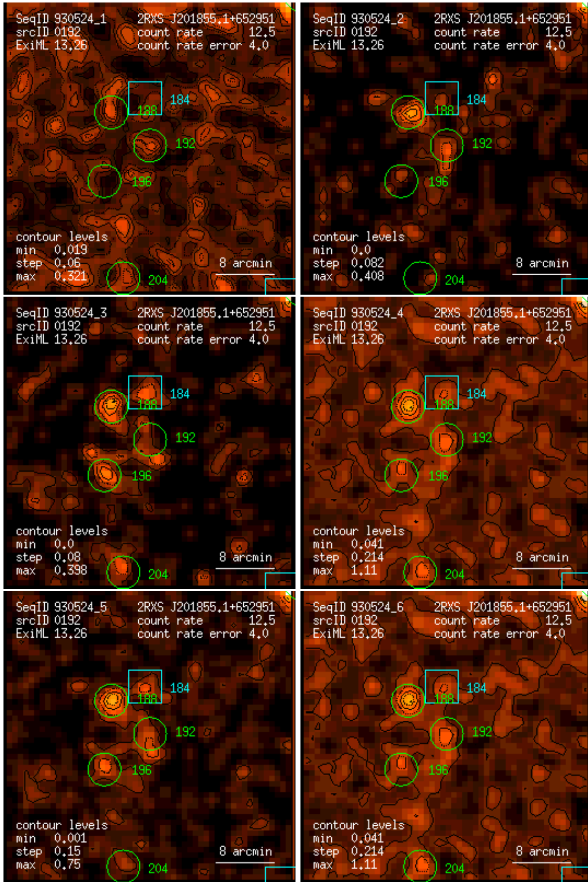
Figure 192: RASS 930524: detection 0192: band rate images, Gaussian filter: (1) PSPC channels 11 – 41, (2) 52 – 90, (3) 91 – 201, (4) 11 – 235, (5) 52 – 201, (6) 11 – 201. Broad band rates in counts/ks. Band rate contour levels in counts/ks/arcmin 2 .
