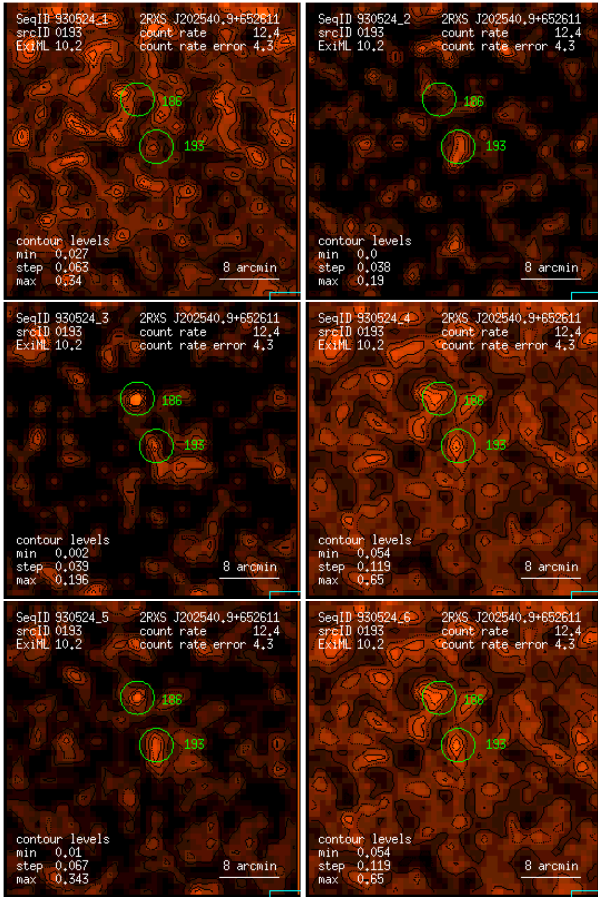
Figure 193: RASS 930524: detection 0193: band rate images, Gaussian filter: (1) PSPC channels 11 – 41, (2) 52 – 90, (3) 91 – 201, (4) 11 – 235, (5) 52 – 201, (6) 11 – 201. Broad band rates in counts/ks. Band rate contour levels in counts/ks/arcmin 2 .
