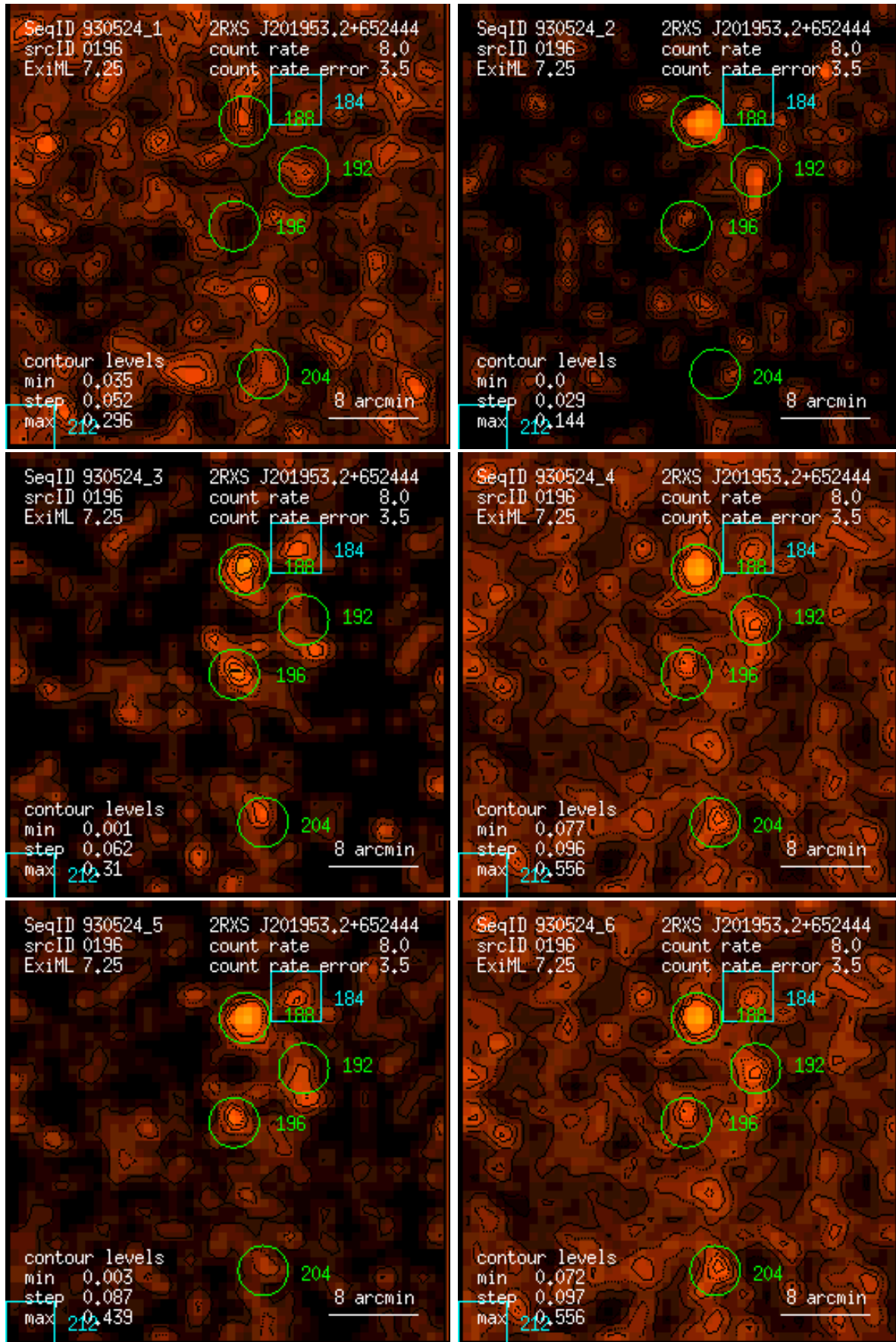
Figure 196: RASS 930524: detection 0196: band rate images, Gaussian filter: (1) PSPC channels 11 – 41, (2) 52 – 90, (3) 91 – 201, (4) 11 – 235, (5) 52 – 201, (6) 11 – 201. Broad band rates in counts/ks. Band rate contour levels in counts/ks/arcmin 2 .
