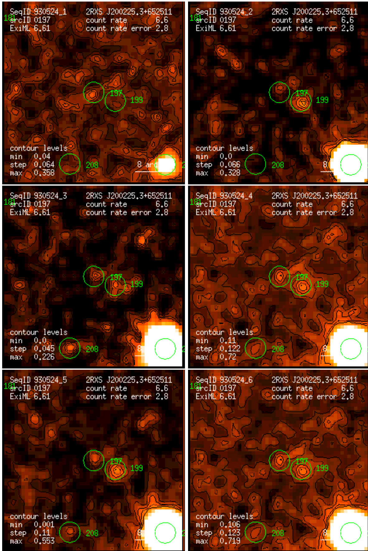
Figure 197: RASS 930524: detection 0197: band rate images, Gaussian filter: (1) PSPC channels 11 – 41, (2) 52 – 90, (3) 91 – 201, (4) 11 – 235, (5) 52 – 201, (6) 11 – 201. Broad band rates in counts/ks. Band rate contour levels in counts/ks/arcmin 2 .
