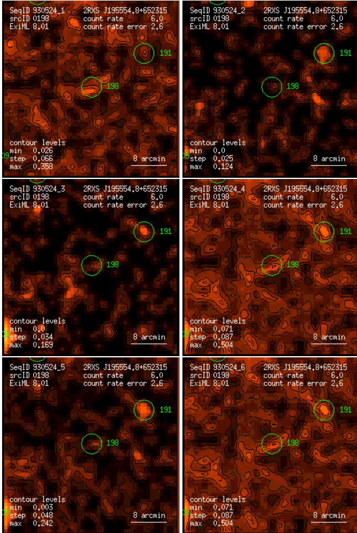
Figure 198: RASS 930524: detection 0198: band rate images, Gaussian filter: (1) PSPC channels 11 – 41, (2) 52 – 90, (3) 91 – 201, (4) 11 – 235, (5) 52 – 201, (6) 11 – 201. Broad band rates in counts/ks. Band rate contour levels in counts/ks/arcmin 2 .
