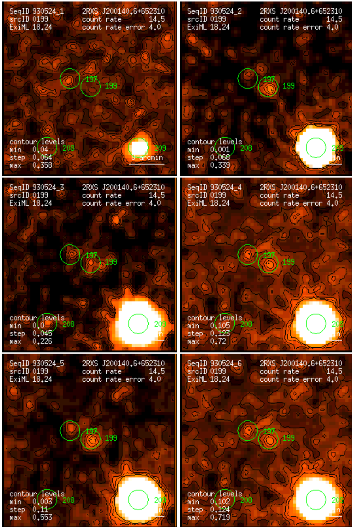
Figure 199: RASS 930524: detection 0199: band rate images, Gaussian filter: (1) PSPC channels 11 – 41, (2) 52 – 90, (3) 91 – 201, (4) 11 – 235, (5) 52 – 201, (6) 11 – 201. Broad band rates in counts/ks. Band rate contour levels in counts/ks/arcmin 2 .
