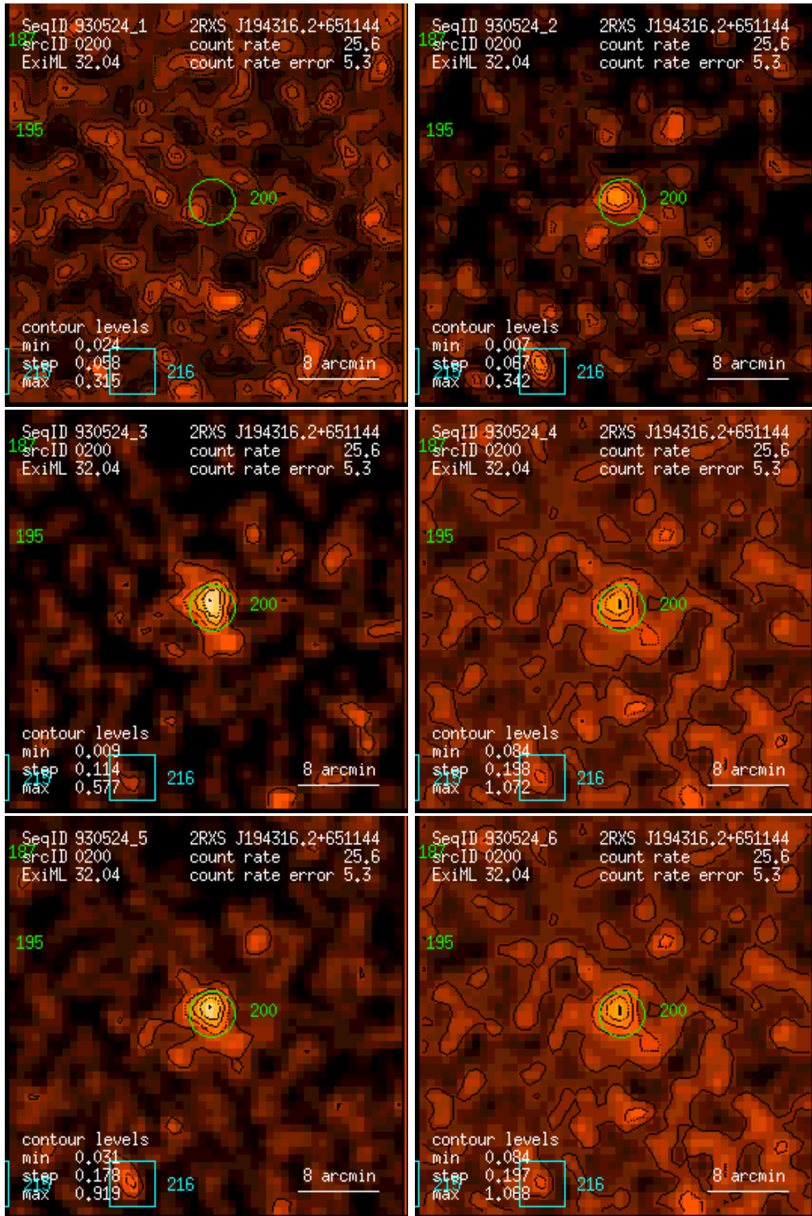
Figure 200: RASS 930524: detection 0200: band rate images, Gaussian filter: (1) PSPC channels 11 – 41, (2) 52 – 90, (3) 91 – 201, (4) 11 – 235, (5) 52 – 201, (6) 11 – 201. Broad band rates in counts/ks. Band rate contour levels in counts/ks/arcmin 2 .
