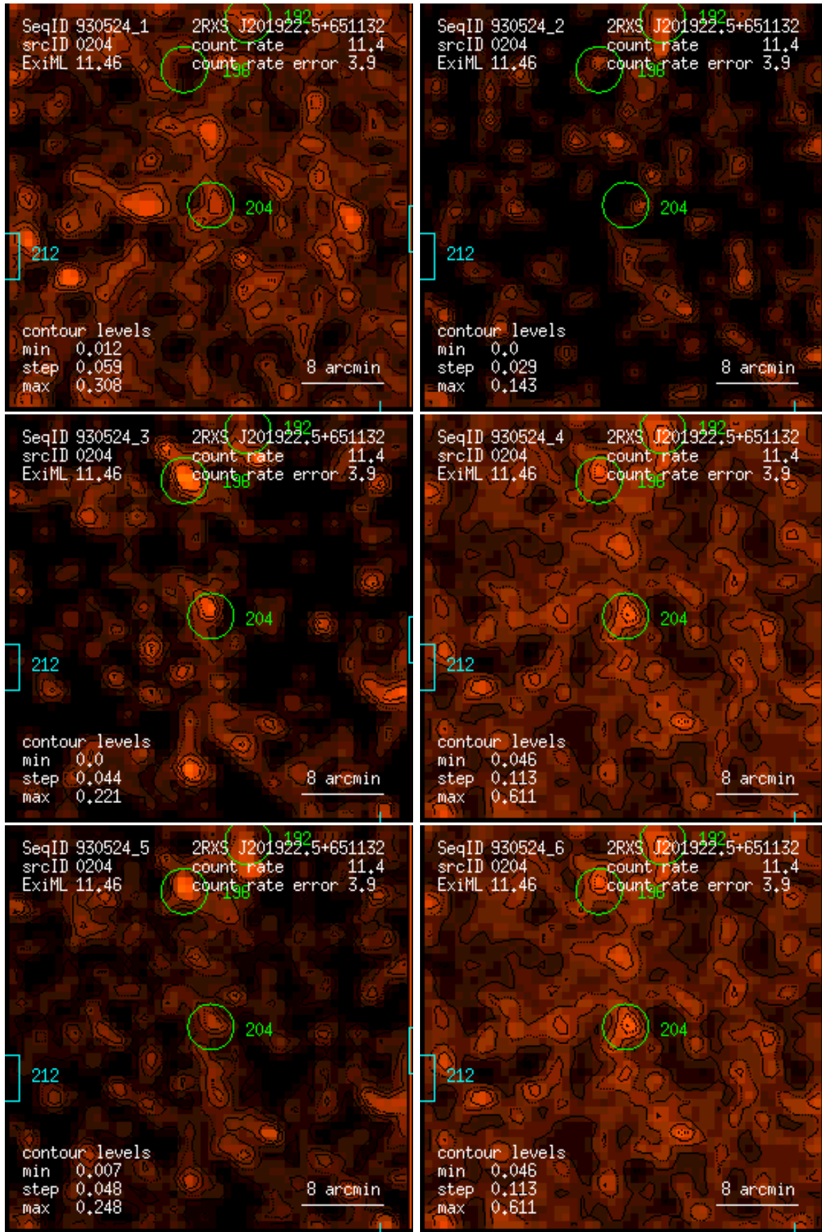
Figure 204: RASS 930524: detection 0204: band rate images, Gaussian filter: (1) PSPC channels 11 – 41, (2) 52 – 90, (3) 91 – 201, (4) 11 – 235, (5) 52 – 201, (6) 11 – 201. Broad band rates in counts/ks. Band rate contour levels in counts/ks/arcmin 2 .
