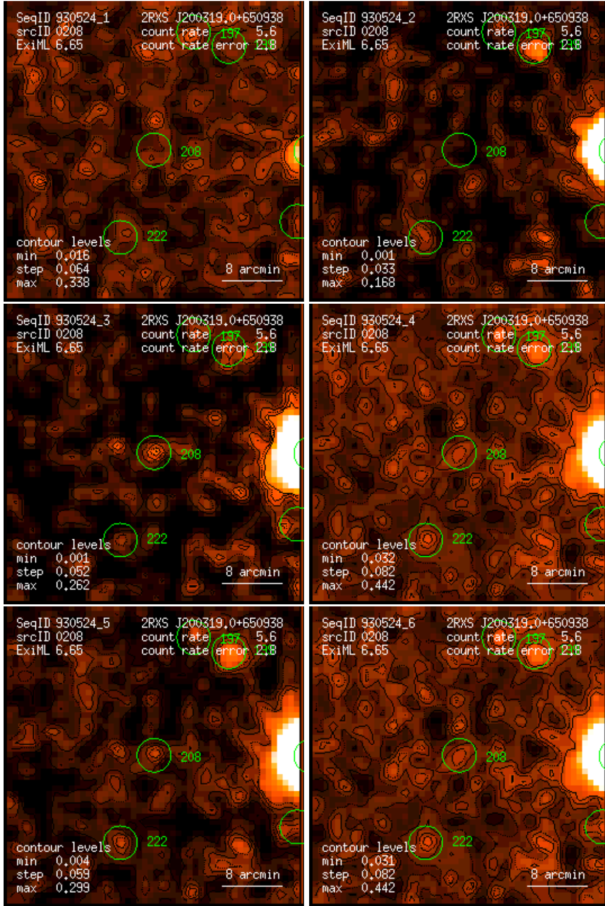
Figure 208: RASS 930524: detection 0208: band rate images, Gaussian filter: (1) PSPC channels 11 – 41, (2) 52 – 90, (3) 91 – 201, (4) 11 – 235, (5) 52 – 201, (6) 11 – 201. Broad band rates in counts/ks. Band rate contour levels in counts/ks/arcmin 2 .
