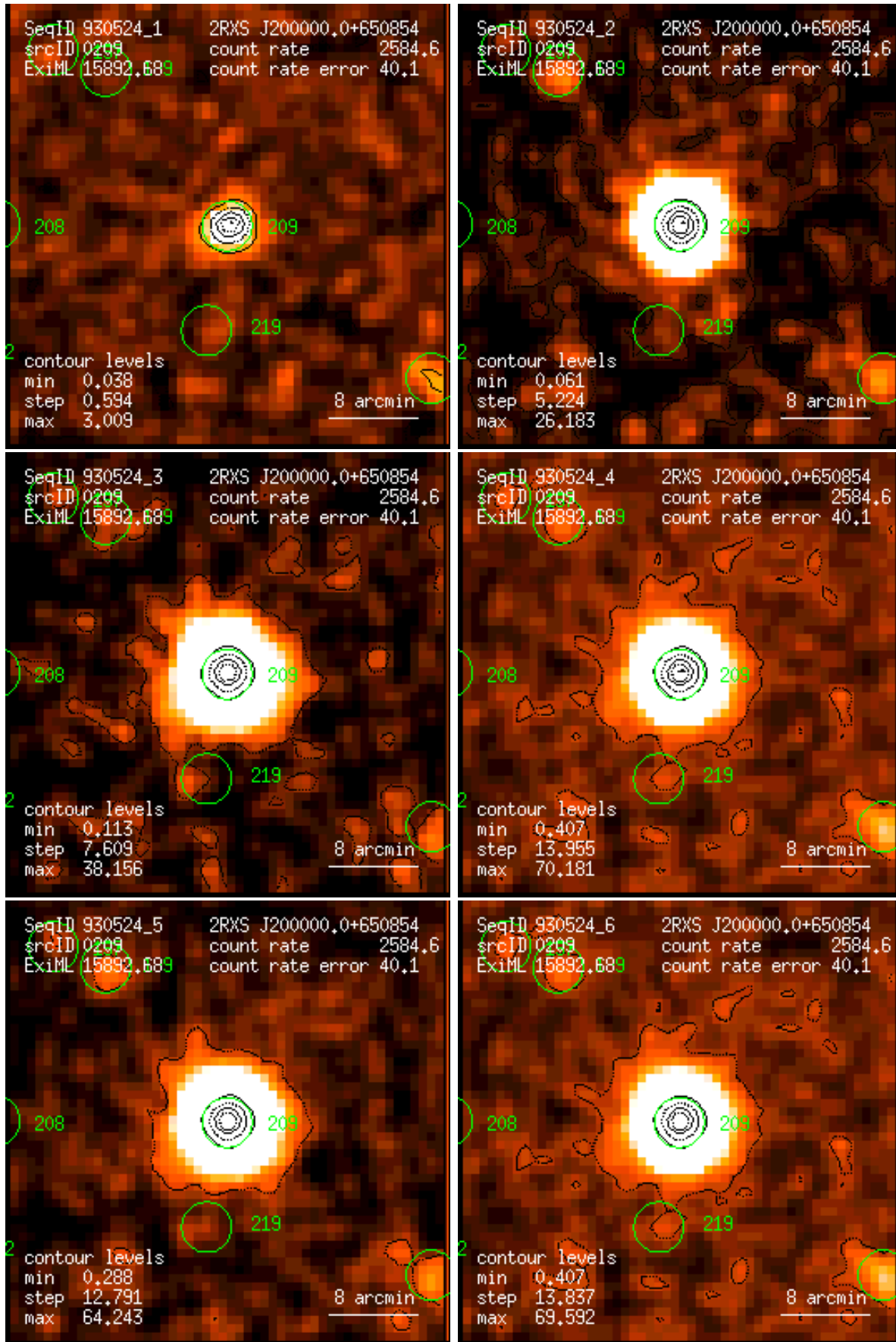
Figure 209: RASS 930524: detection 0209: band rate images, Gaussian filter: (1) PSPC channels 11 – 41, (2) 52 – 90, (3) 91 – 201, (4) 11 – 235, (5) 52 – 201, (6) 11 – 201. Broad band rates in counts/ks. Band rate contour levels in counts/ks/arcmin 2 .
