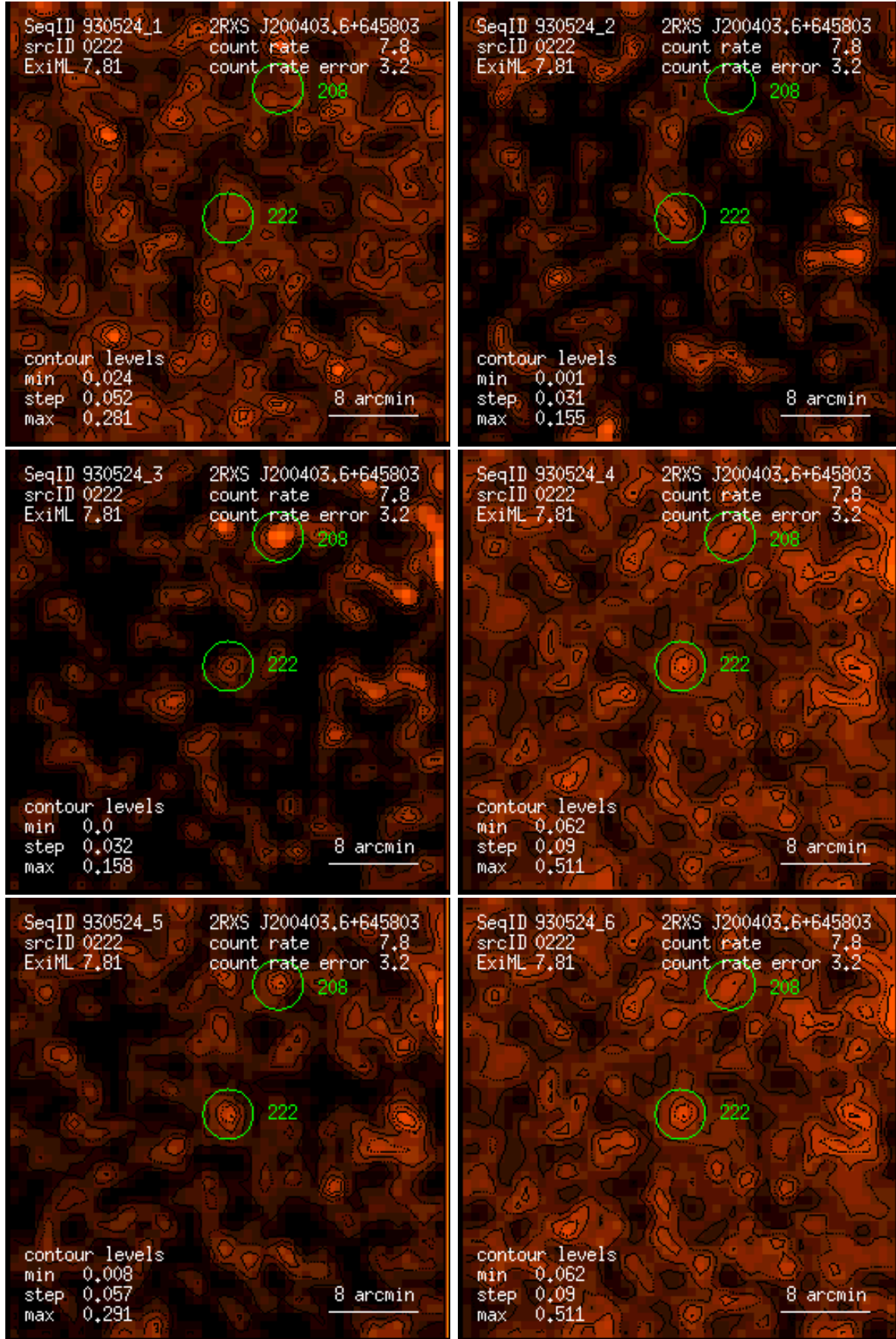
Figure 222: RASS 930524: detection 0222: band rate images, Gaussian filter: (1) PSPC channels 11 – 41, (2) 52 – 90, (3) 91 – 201, (4) 11 – 235, (5) 52 – 201, (6) 11 – 201. Broad band rates in counts/ks. Band rate contour levels in counts/ks/arcmin 2 .
