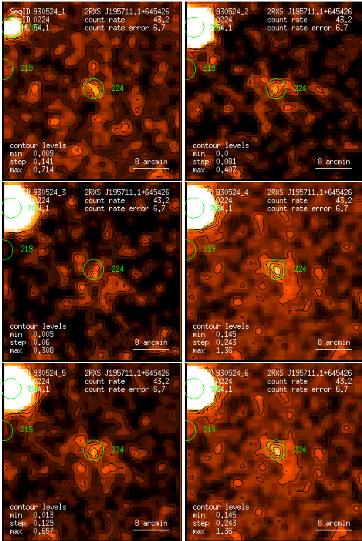
Figure 224: RASS 930524: detection 0224: band rate images, Gaussian filter: (1) PSPC channels 11 – 41, (2) 52 – 90, (3) 91 – 201, (4) 11 – 235, (5) 52 – 201, (6) 11 – 201. Broad band rates in counts/ks. Band rate contour levels in counts/ks/arcmin 2 .
