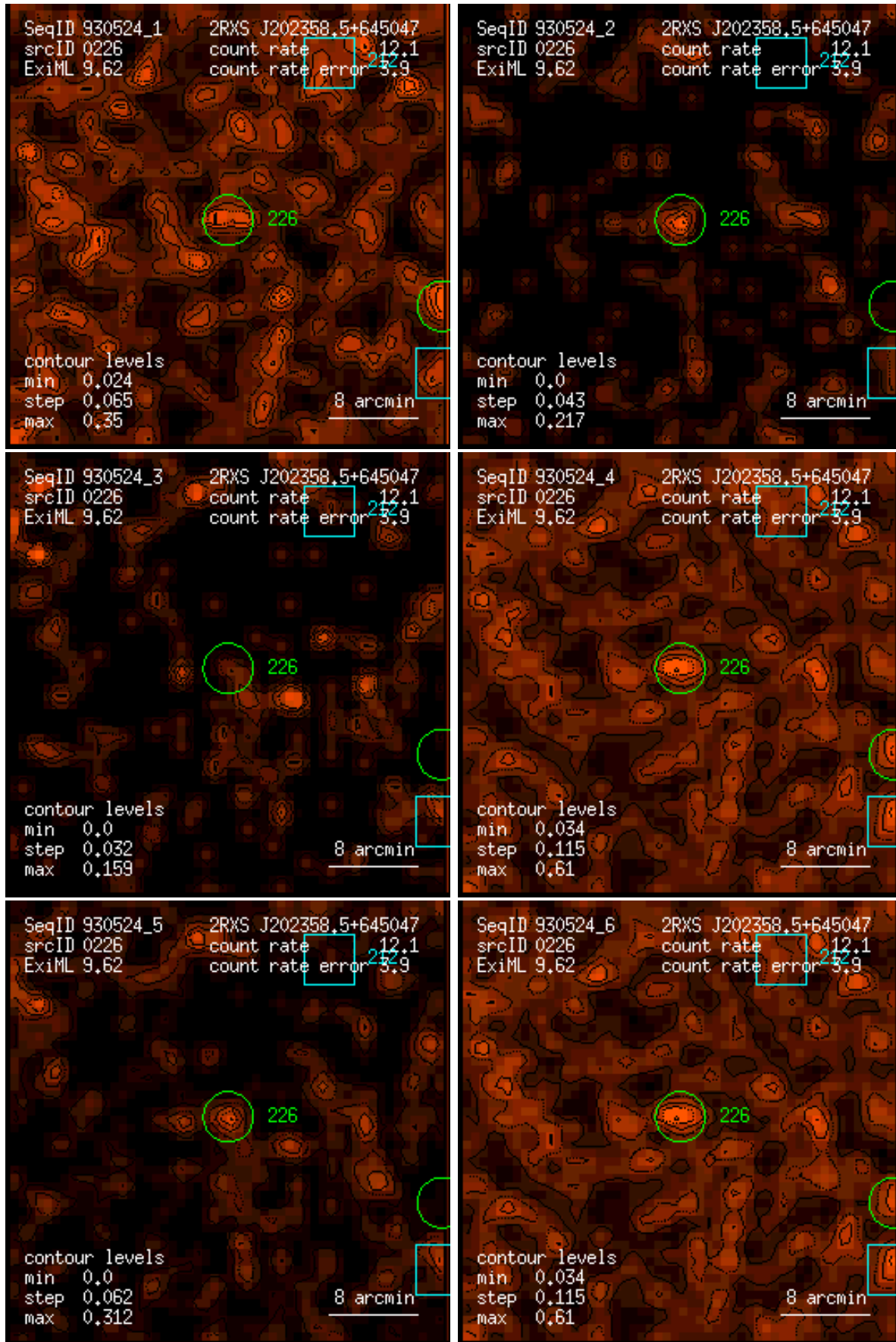
Figure 226: RASS 930524: detection 0226: band rate images, Gaussian filter: (1) PSPC channels 11 – 41, (2) 52 – 90, (3) 91 – 201, (4) 11 – 235, (5) 52 – 201, (6) 11 – 201. Broad band rates in counts/ks. Band rate contour levels in counts/ks/arcmin 2 .
