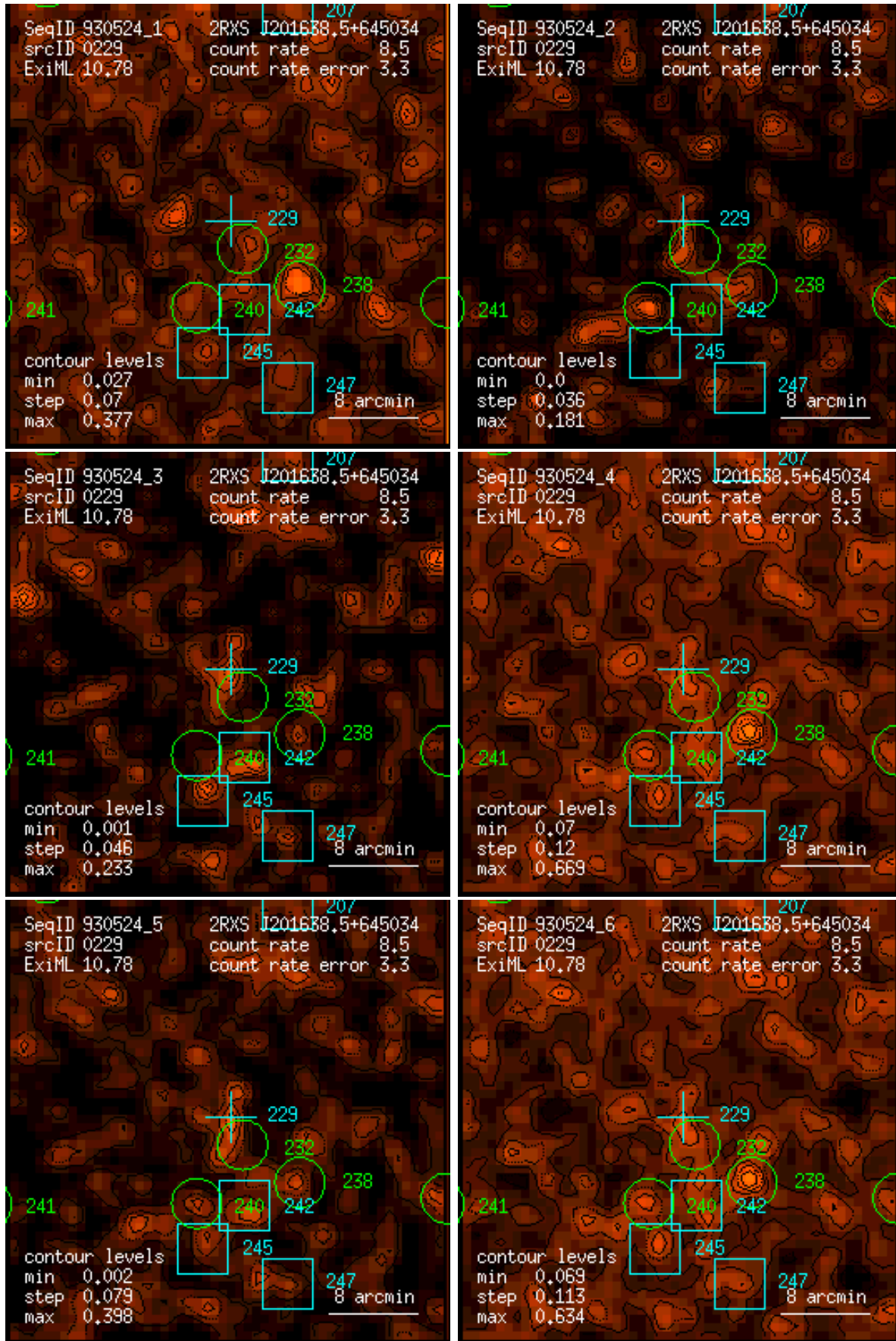
Figure 229: RASS 930524: detection 0229: band rate images, Gaussian filter: (1) PSPC channels 11 – 41, (2) 52 – 90, (3) 91 – 201, (4) 11 – 235, (5) 52 – 201, (6) 11 – 201. Broad band rates in counts/ks. Band rate contour levels in counts/ks/arcmin 2 .
