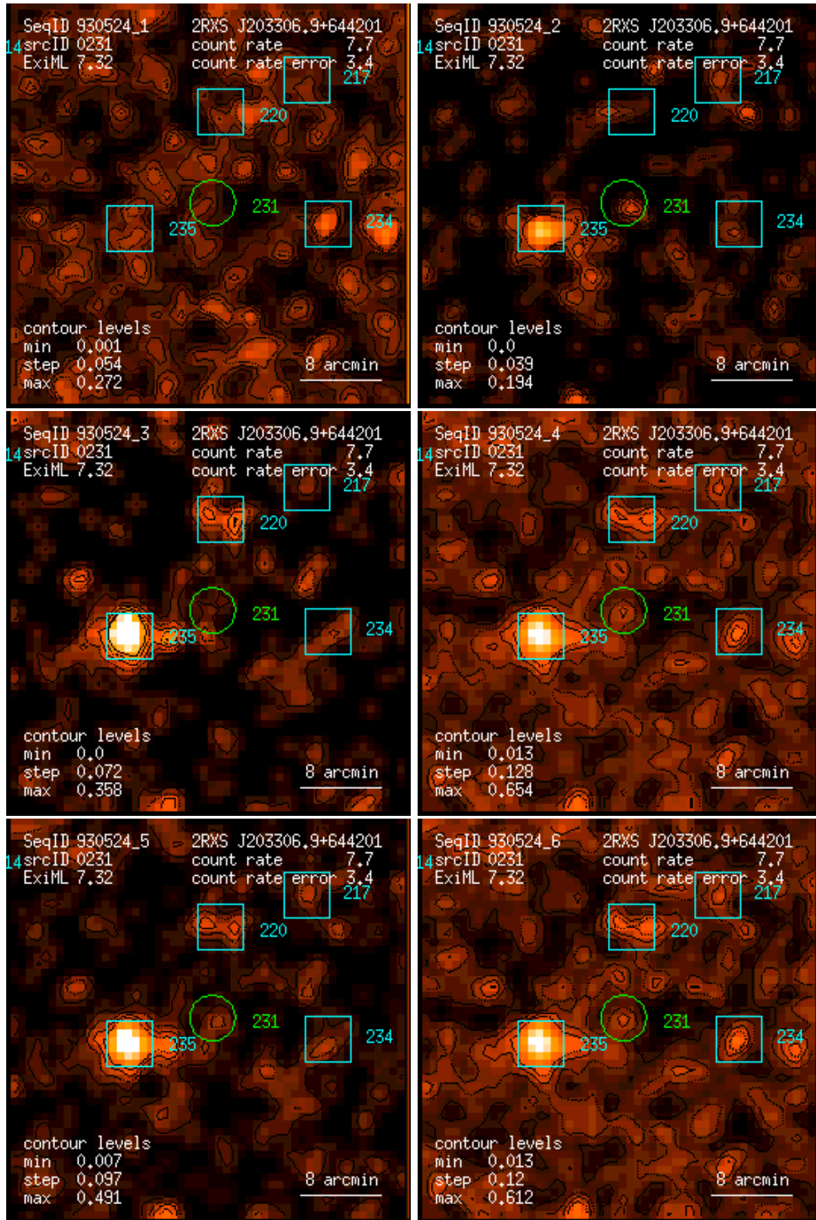
Figure 231: RASS 930524: detection 0231: band rate images, Gaussian filter: (1) PSPC channels 11 – 41, (2) 52 – 90, (3) 91 – 201, (4) 11 – 235, (5) 52 – 201, (6) 11 – 201. Broad band rates in counts/ks. Band rate contour levels in counts/ks/arcmin 2 .
