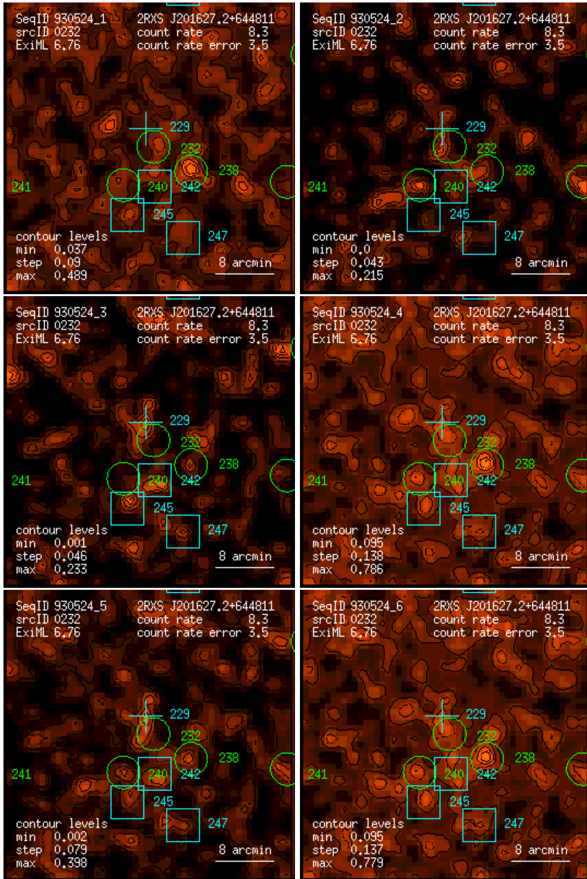
Figure 232: RASS 930524: detection 0232: band rate images, Gaussian filter: (1) PSPC channels 11 – 41, (2) 52 – 90, (3) 91 – 201, (4) 11 – 235, (5) 52 – 201, (6) 11 – 201. Broad band rates in counts/ks. Band rate contour levels in counts/ks/arcmin 2 .
