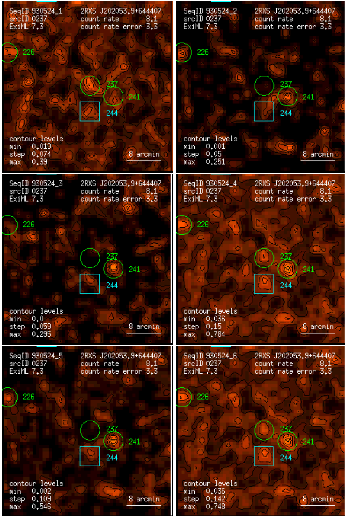
Figure 237: RASS 930524: detection 0237: band rate images, Gaussian filter: (1) PSPC channels 11 – 41, (2) 52 – 90, (3) 91 – 201, (4) 11 – 235, (5) 52 – 201, (6) 11 – 201. Broad band rates in counts/ks. Band rate contour levels in counts/ks/arcmin 2 .
