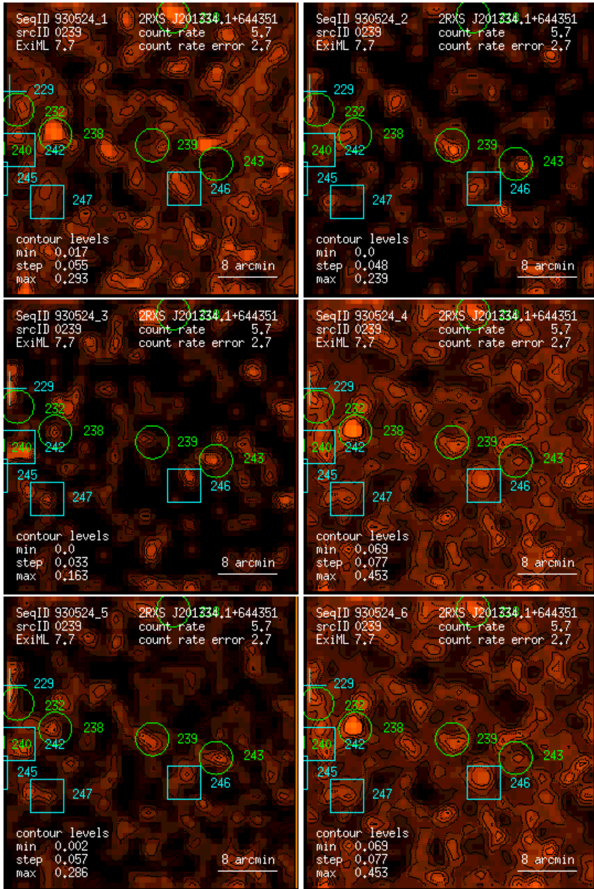
Figure 239: RASS 930524: detection 0239: band rate images, Gaussian filter: (1) PSPC channels 11 – 41, (2) 52 – 90, (3) 91 – 201, (4) 11 – 235, (5) 52 – 201, (6) 11 – 201. Broad band rates in counts/ks. Band rate contour levels in counts/ks/arcmin 2 .
