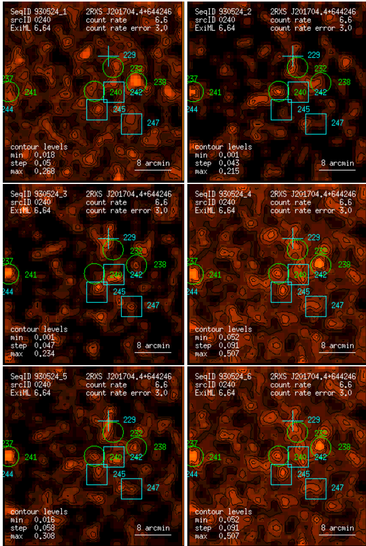
Figure 240: RASS 930524: detection 0240: band rate images, Gaussian filter: (1) PSPC channels 11 – 41, (2) 52 – 90, (3) 91 – 201, (4) 11 – 235, (5) 52 – 201, (6) 11 – 201. Broad band rates in counts/ks. Band rate contour levels in counts/ks/arcmin 2 .
