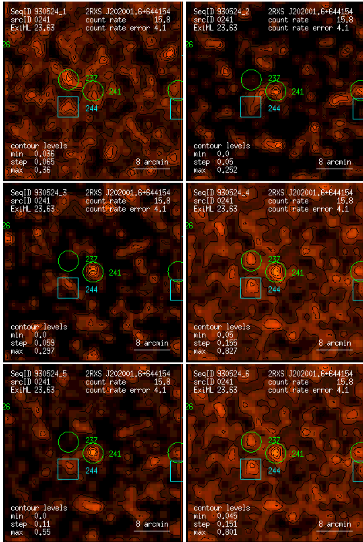
Figure 241: RASS 930524: detection 0241: band rate images, Gaussian filter: (1) PSPC channels 11 – 41, (2) 52 – 90, (3) 91 – 201, (4) 11 – 235, (5) 52 – 201, (6) 11 – 201. Broad band rates in counts/ks. Band rate contour levels in counts/ks/arcmin 2 .
