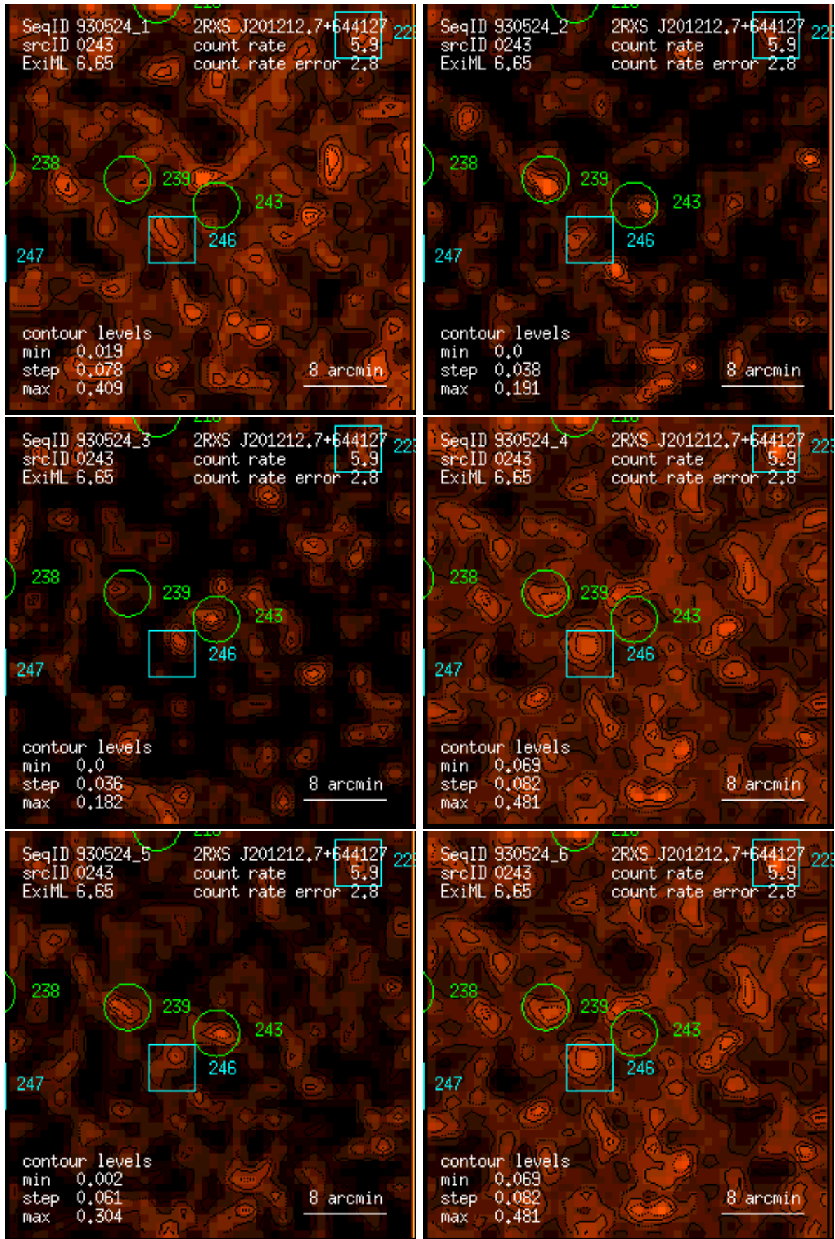
Figure 243: RASS 930524: detection 0243: band rate images, Gaussian filter: (1) PSPC channels 11 – 41, (2) 52 – 90, (3) 91 – 201, (4) 11 – 235, (5) 52 – 201, (6) 11 – 201. Broad band rates in counts/ks. Band rate contour levels in counts/ks/arcmin 2 .
