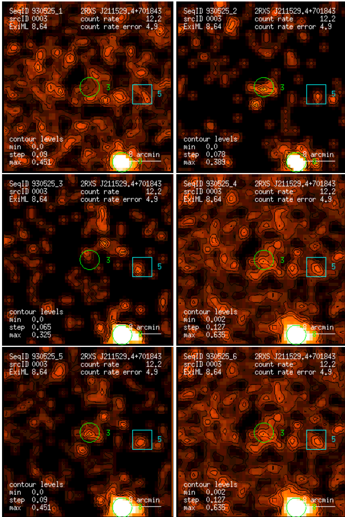
Figure 3: RASS 930525: detection 0003: band rate images, Gaussian filter: (1) PSPC channels 11 – 41, (2) 52 – 90, (3) 91 – 201, (4) 11 – 235, (5) 52 – 201, (6) 11 – 201. Broad band rates in counts/ks. Band rate contour levels in counts/ks/arcmin 2 .
