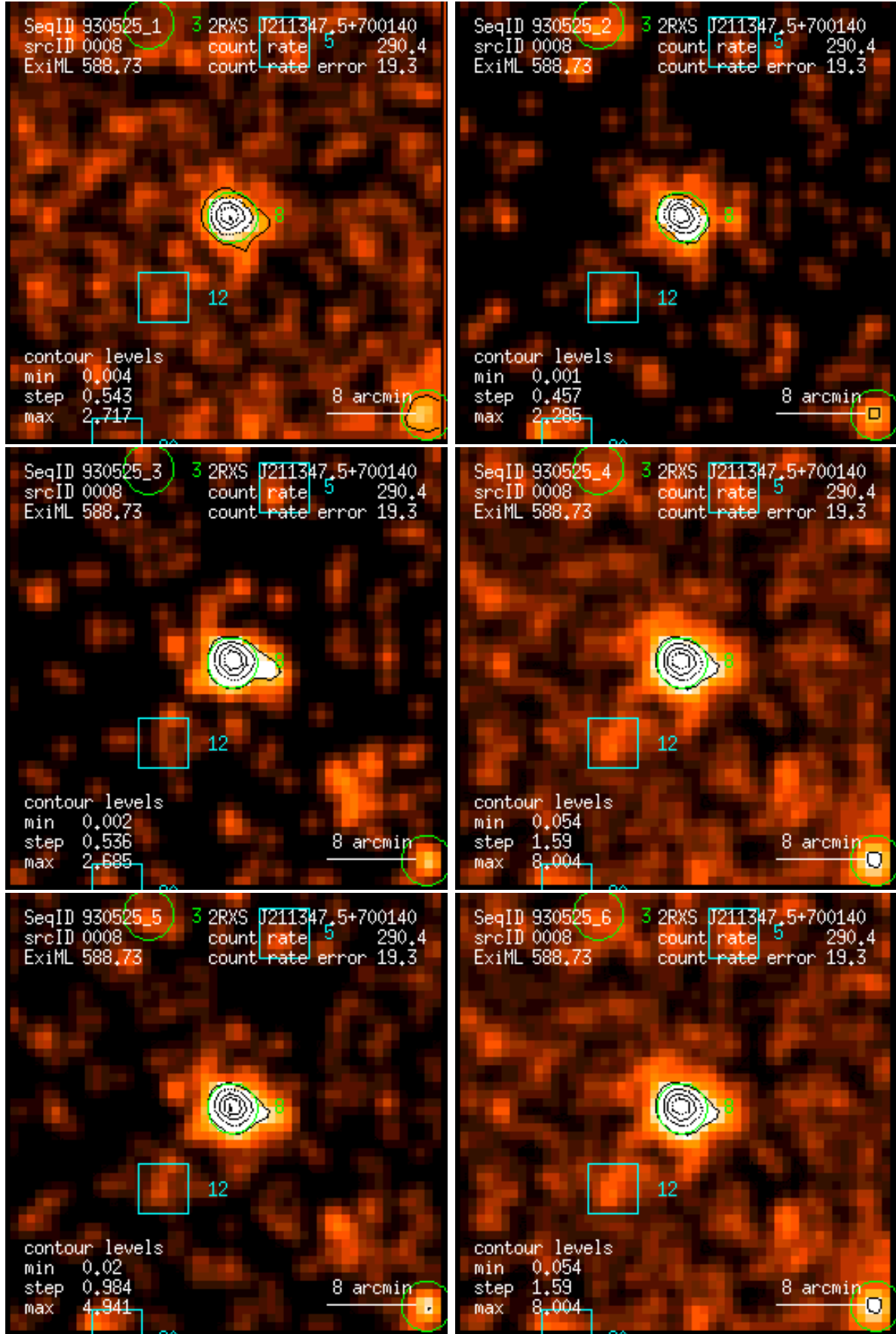
Figure 8: RASS 930525: detection 0008: band rate images, Gaussian filter: (1) PSPC channels 11 – 41, (2) 52 – 90, (3) 91 – 201, (4) 11 – 235, (5) 52 – 201, (6) 11 – 201. Broad band rates in counts/ks. Band rate contour levels in counts/ks/arcmin 2 .
