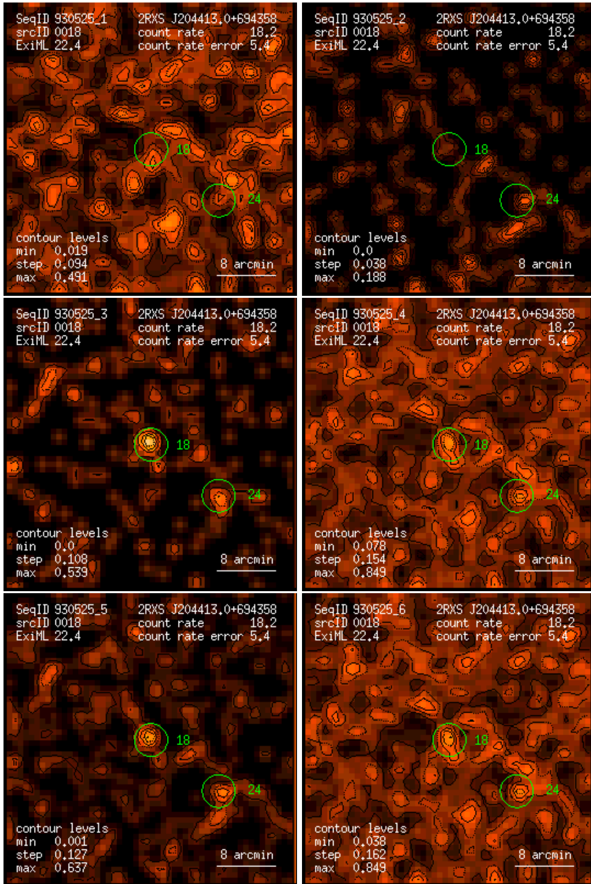
Figure 18: RASS 930525: detection 0018: band rate images, Gaussian filter: (1) PSPC channels 11 – 41, (2) 52 – 90, (3) 91 – 201, (4) 11 – 235, (5) 52 – 201, (6) 11 – 201. Broad band rates in counts/ks. Band rate contour levels in counts/ks/arcmin 2 .
