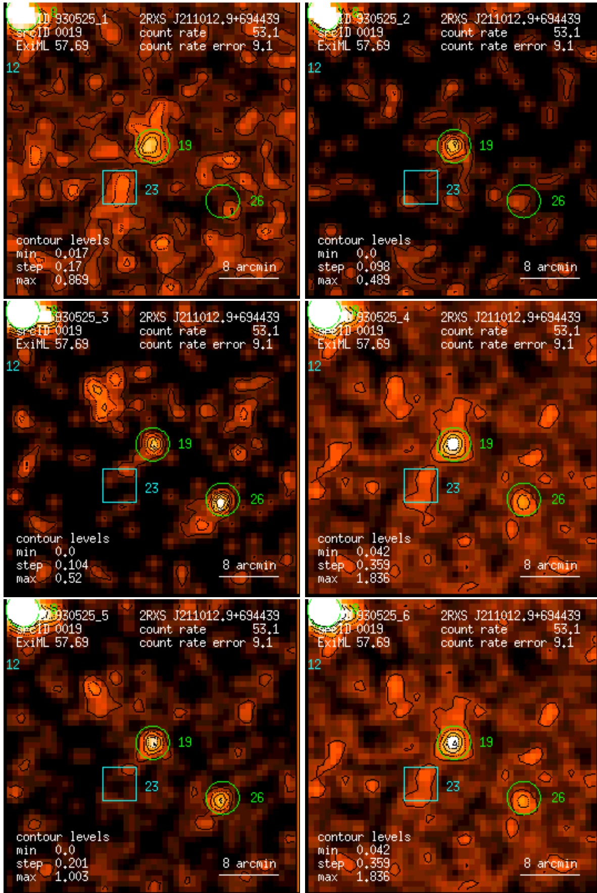
Figure 19: RASS 930525: detection 0019: band rate images, Gaussian filter: (1) PSPC channels 11 – 41, (2) 52 – 90, (3) 91 – 201, (4) 11 – 235, (5) 52 – 201, (6) 11 – 201. Broad band rates in counts/ks. Band rate contour levels in counts/ks/arcmin 2 .
