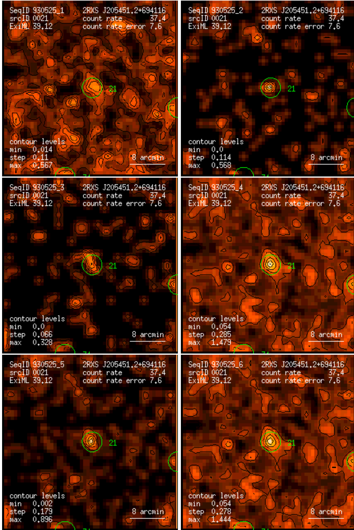
Figure 21: RASS 930525: detection 0021: band rate images, Gaussian filter: (1) PSPC channels 11 – 41, (2) 52 – 90, (3) 91 – 201, (4) 11 – 235, (5) 52 – 201, (6) 11 – 201. Broad band rates in counts/ks. Band rate contour levels in counts/ks/arcmin 2 .
