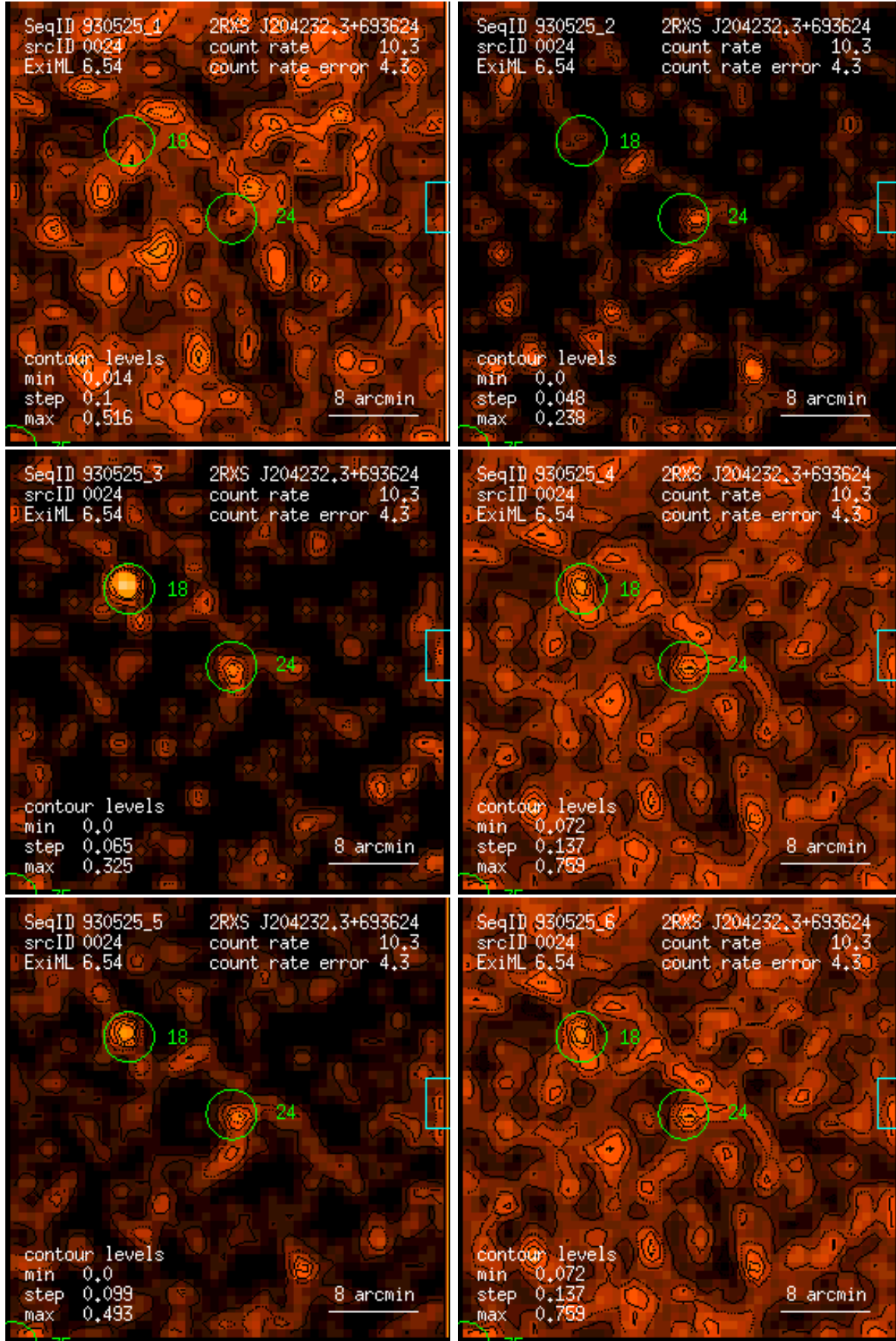
Figure 24: RASS 930525: detection 0024: band rate images, Gaussian filter: (1) PSPC channels 11 – 41, (2) 52 – 90, (3) 91 – 201, (4) 11 – 235, (5) 52 – 201, (6) 11 – 201. Broad band rates in counts/ks. Band rate contour levels in counts/ks/arcmin 2 .
