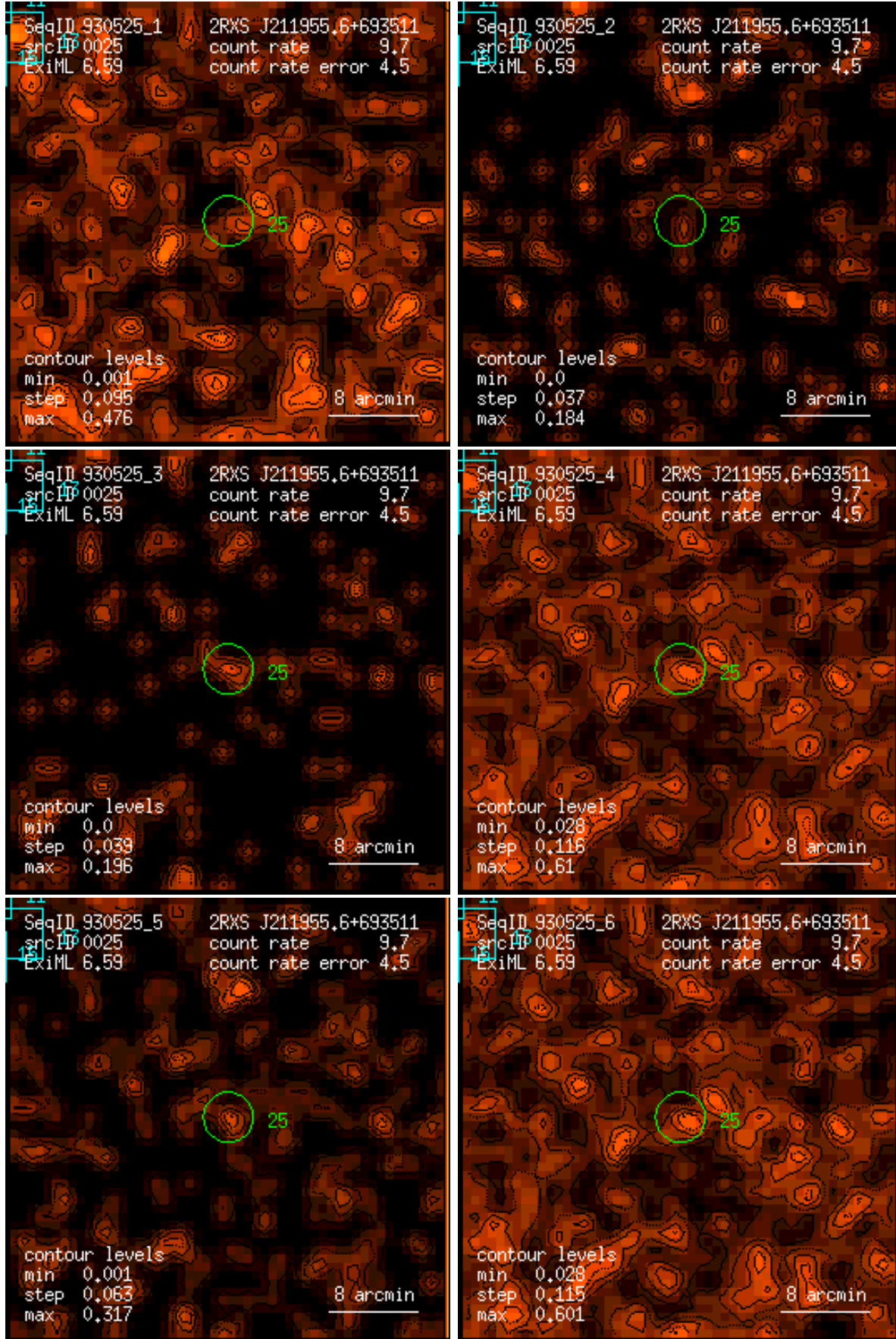
Figure 25: RASS 930525: detection 0025: band rate images, Gaussian filter: (1) PSPC channels 11 – 41, (2) 52 – 90, (3) 91 – 201, (4) 11 – 235, (5) 52 – 201, (6) 11 – 201. Broad band rates in counts/ks. Band rate contour levels in counts/ks/arcmin 2 .
