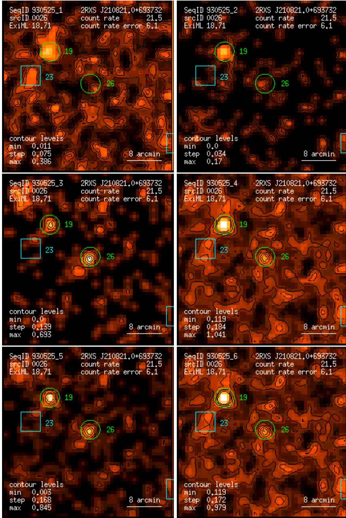
Figure 26: RASS 930525: detection 0026: band rate images, Gaussian filter: (1) PSPC channels 11 – 41, (2) 52 – 90, (3) 91 – 201, (4) 11 – 235, (5) 52 – 201, (6) 11 – 201. Broad band rates in counts/ks. Band rate contour levels in counts/ks/arcmin 2 .
