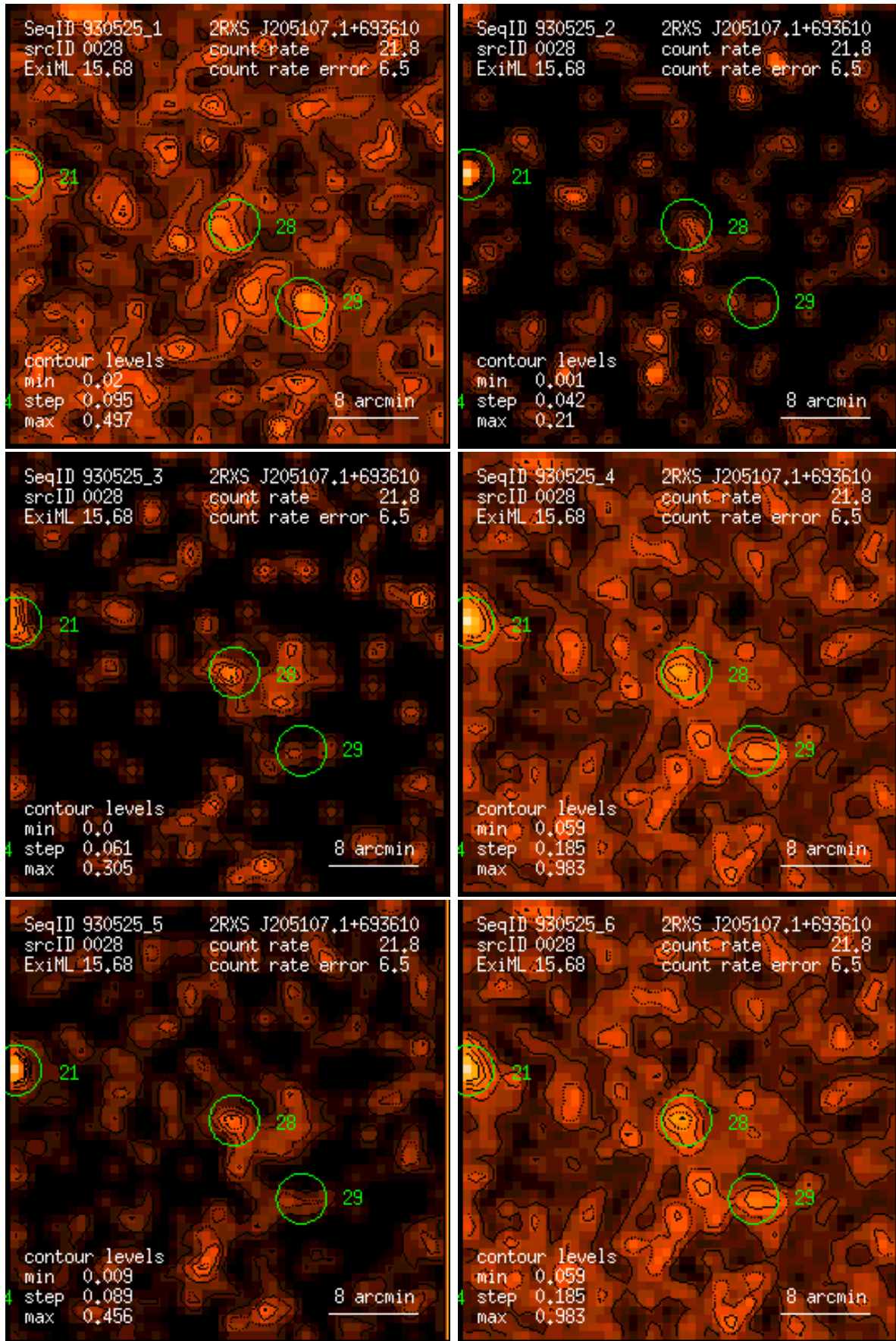
Figure 28: RASS 930525: detection 0028: band rate images, Gaussian filter: (1) PSPC channels 11 – 41, (2) 52 – 90, (3) 91 – 201, (4) 11 – 235, (5) 52 – 201, (6) 11 – 201. Broad band rates in counts/ks. Band rate contour levels in counts/ks/arcmin 2 .
