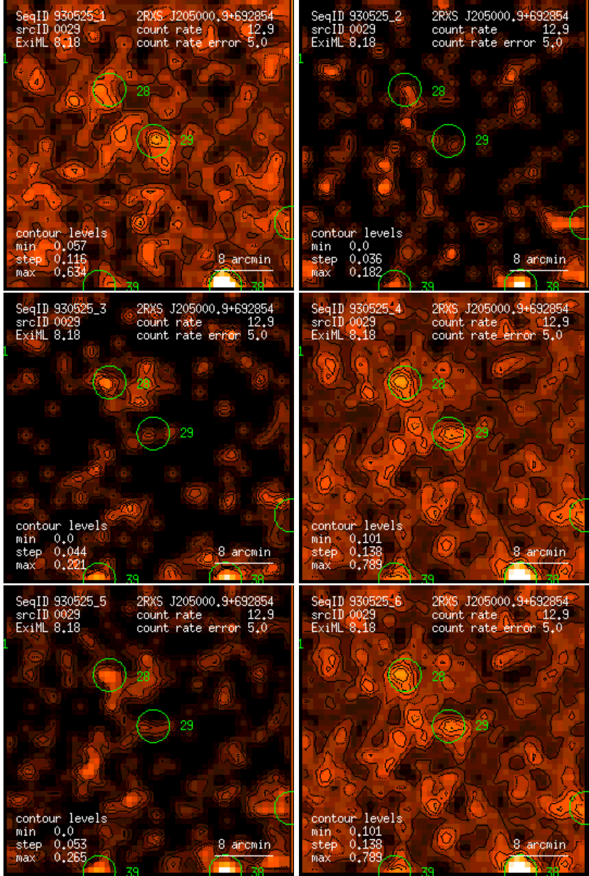
Figure 29: RASS 930525: detection 0029: band rate images, Gaussian filter: (1) PSPC channels 11 – 41, (2) 52 – 90, (3) 91 – 201, (4) 11 – 235, (5) 52 – 201, (6) 11 – 201. Broad band rates in counts/ks. Band rate contour levels in counts/ks/arcmin 2 .
