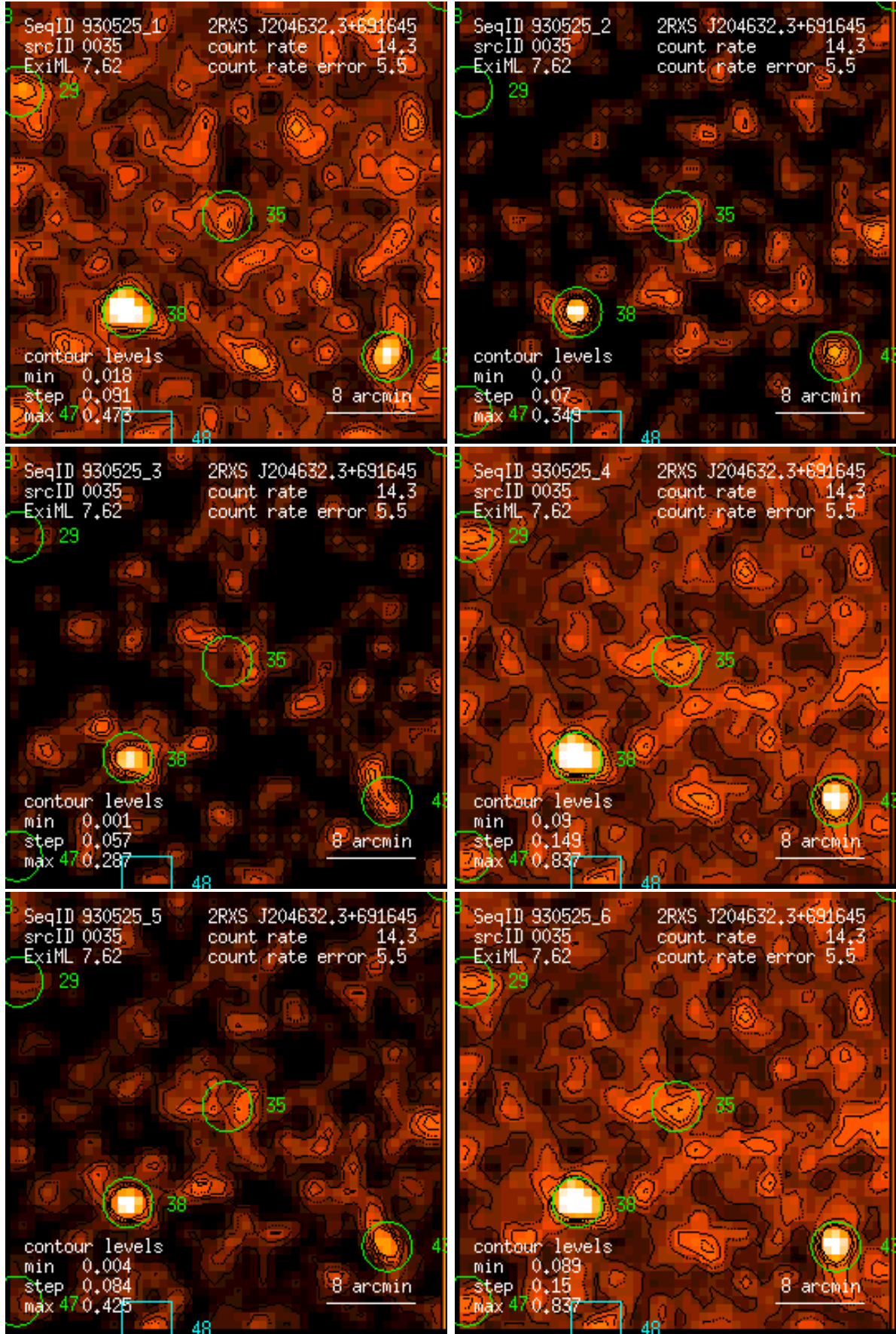
Figure 35: RASS 930525: detection 0035: band rate images, Gaussian filter: (1) PSPC channels 11 – 41, (2) 52 – 90, (3) 91 – 201, (4) 11 – 235, (5) 52 – 201, (6) 11 – 201. Broad band rates in counts/ks. Band rate contour levels in counts/ks/arcmin 2 .
