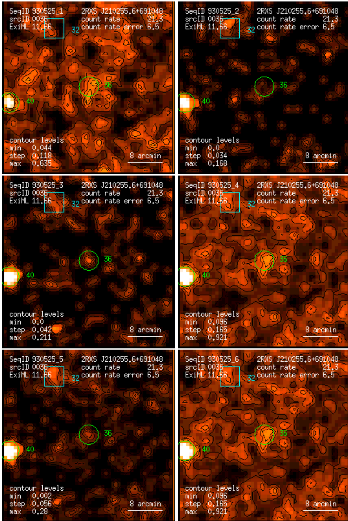
Figure 36: RASS 930525: detection 0036: band rate images, Gaussian filter: (1) PSPC channels 11 – 41, (2) 52 – 90, (3) 91 – 201, (4) 11 – 235, (5) 52 – 201, (6) 11 – 201. Broad band rates in counts/ks. Band rate contour levels in counts/ks/arcmin 2 .
