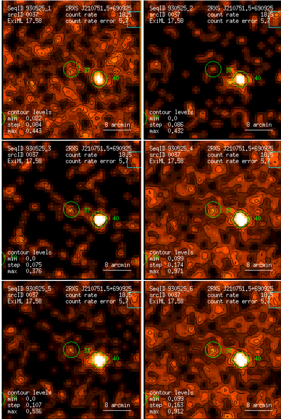
Figure 37: RASS 930525: detection 0037: band rate images, Gaussian filter: (1) PSPC channels 11 – 41, (2) 52 – 90, (3) 91 – 201, (4) 11 – 235, (5) 52 – 201, (6) 11 – 201. Broad band rates in counts/ks. Band rate contour levels in counts/ks/arcmin 2 .
