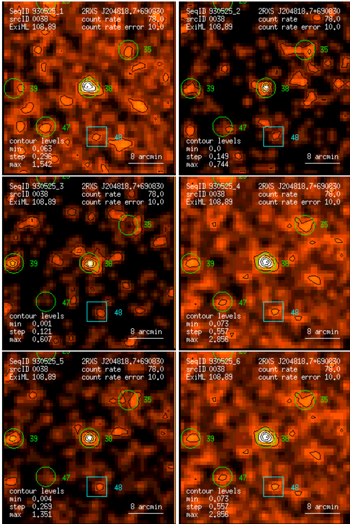
Figure 38: RASS 930525: detection 0038: band rate images, Gaussian filter: (1) PSPC channels 11 – 41, (2) 52 – 90, (3) 91 – 201, (4) 11 – 235, (5) 52 – 201, (6) 11 – 201. Broad band rates in counts/ks. Band rate contour levels in counts/ks/arcmin 2 .
