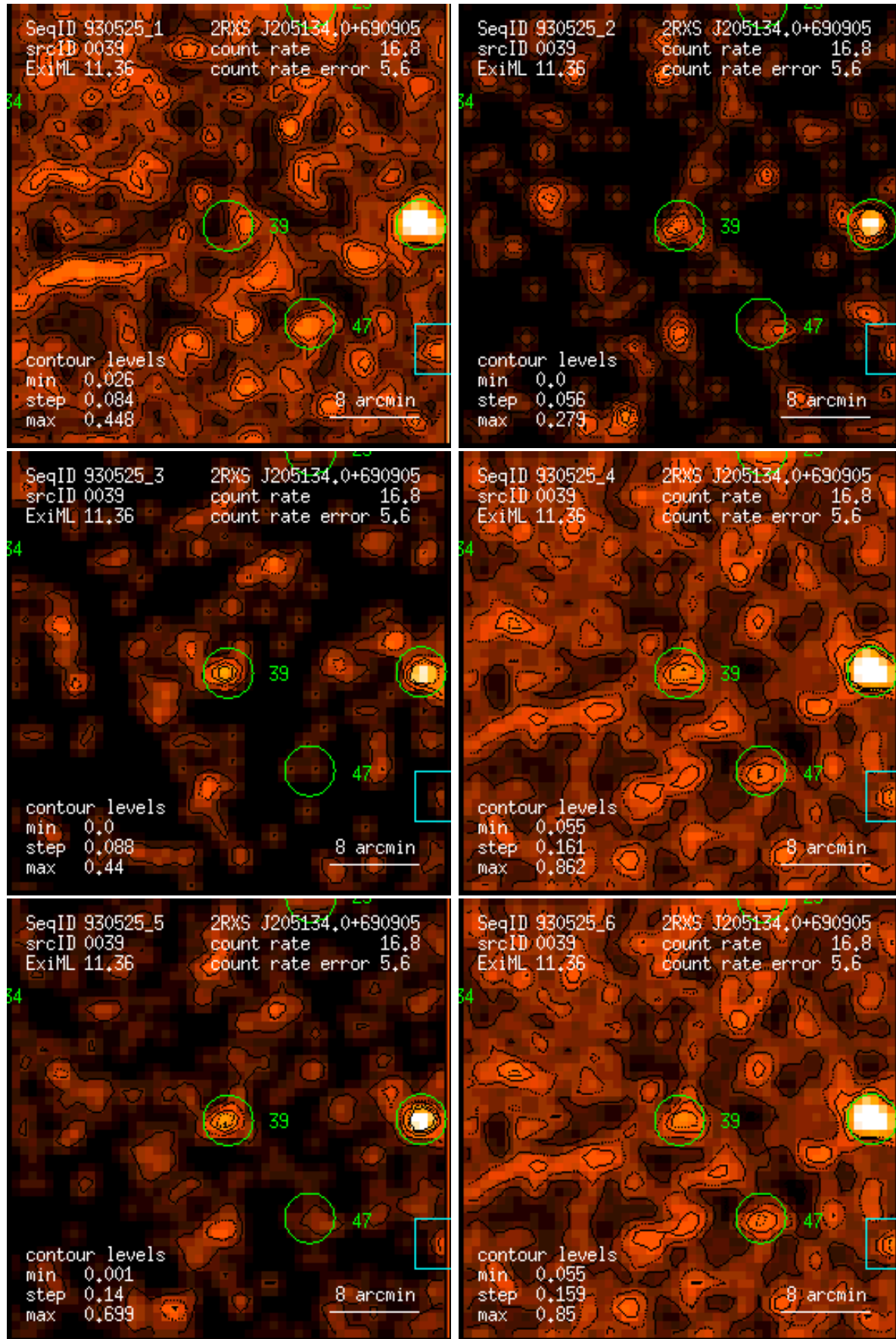
Figure 39: RASS 930525: detection 0039: band rate images, Gaussian filter: (1) PSPC channels 11 – 41, (2) 52 – 90, (3) 91 – 201, (4) 11 – 235, (5) 52 – 201, (6) 11 – 201. Broad band rates in counts/ks. Band rate contour levels in counts/ks/arcmin 2 .
