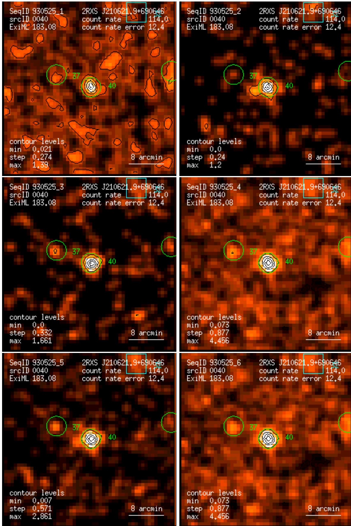
Figure 40: RASS 930525: detection 0040: band rate images, Gaussian filter: (1) PSPC channels 11 – 41, (2) 52 – 90, (3) 91 – 201, (4) 11 – 235, (5) 52 – 201, (6) 11 – 201. Broad band rates in counts/ks. Band rate contour levels in counts/ks/arcmin 2 .
