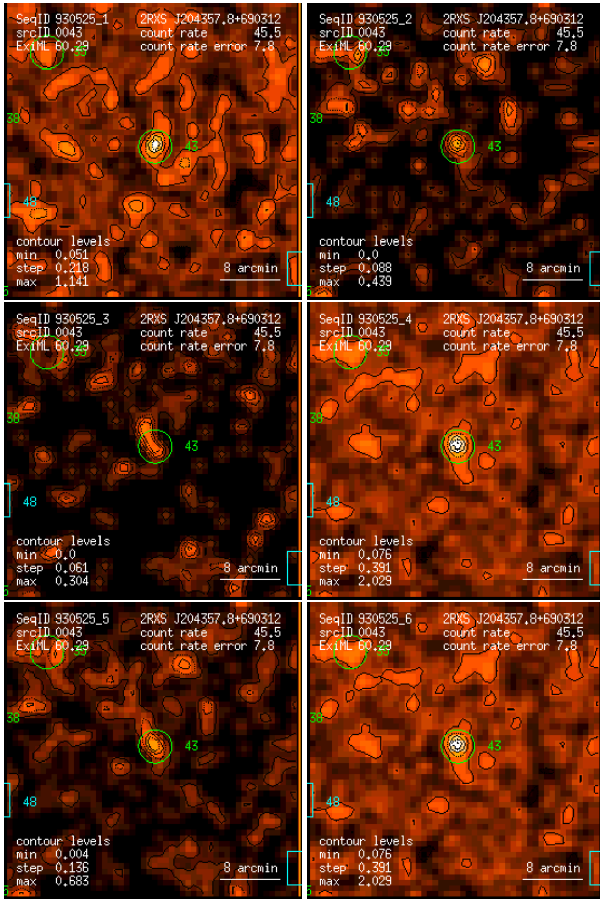
Figure 43: RASS 930525: detection 0043: band rate images, Gaussian filter: (1) PSPC channels 11 – 41, (2) 52 – 90, (3) 91 – 201, (4) 11 – 235, (5) 52 – 201, (6) 11 – 201. Broad band rates in counts/ks. Band rate contour levels in counts/ks/arcmin 2 .
