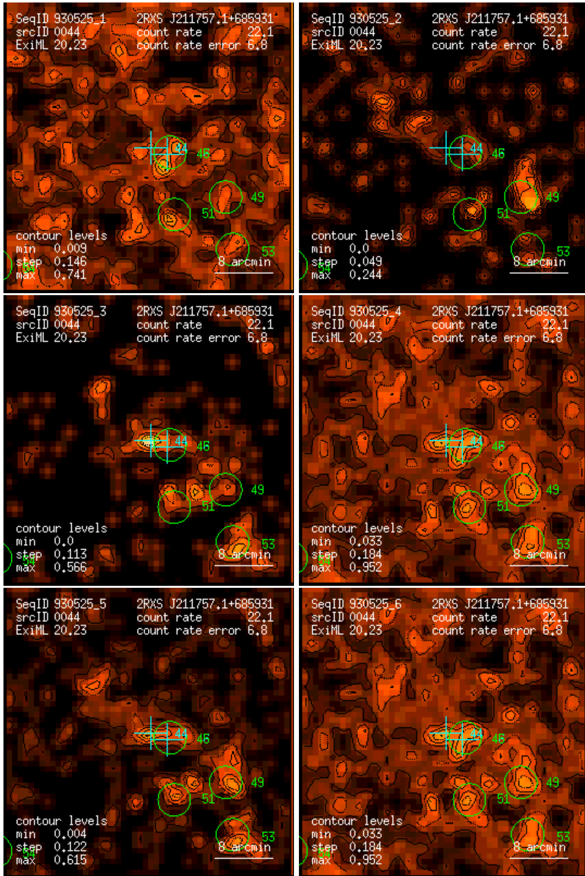
Figure 44: RASS 930525: detection 0044: band rate images, Gaussian filter: (1) PSPC channels 11 – 41, (2) 52 – 90, (3) 91 – 201, (4) 11 – 235, (5) 52 – 201, (6) 11 – 201. Broad band rates in counts/ks. Band rate contour levels in counts/ks/arcmin 2 .
