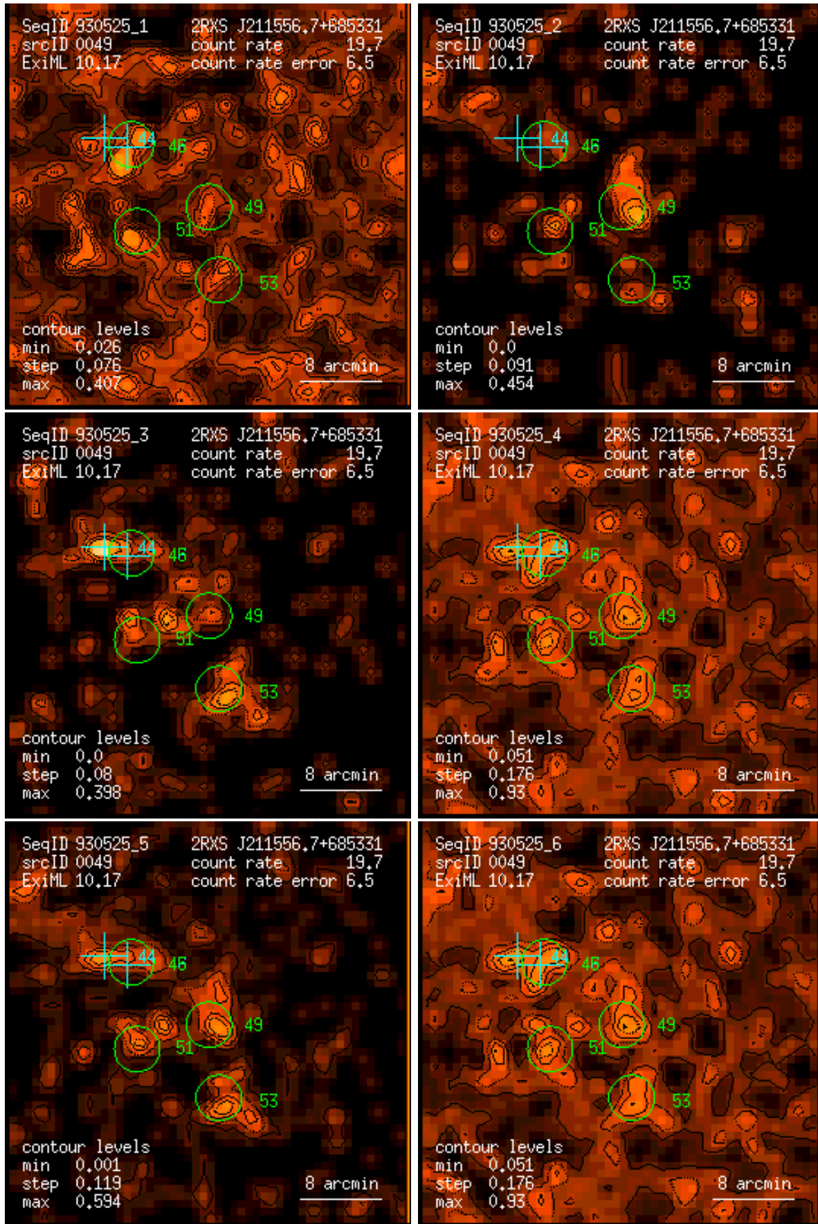
Figure 49: RASS 930525: detection 0049: band rate images, Gaussian filter: (1) PSPC channels 11 – 41, (2) 52 – 90, (3) 91 – 201, (4) 11 – 235, (5) 52 – 201, (6) 11 – 201. Broad band rates in counts/ks. Band rate contour levels in counts/ks/arcmin 2 .
