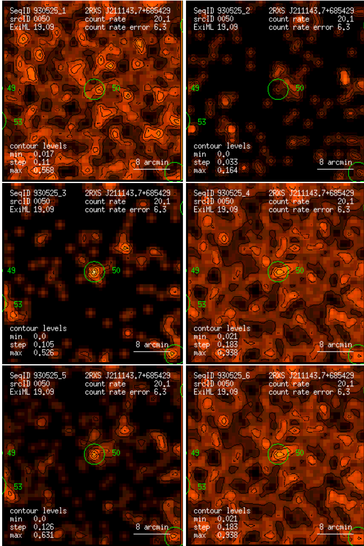
Figure 50: RASS 930525: detection 0050: band rate images, Gaussian filter: (1) PSPC channels 11 – 41, (2) 52 – 90, (3) 91 – 201, (4) 11 – 235, (5) 52 – 201, (6) 11 – 201. Broad band rates in counts/ks. Band rate contour levels in counts/ks/arcmin 2 .
