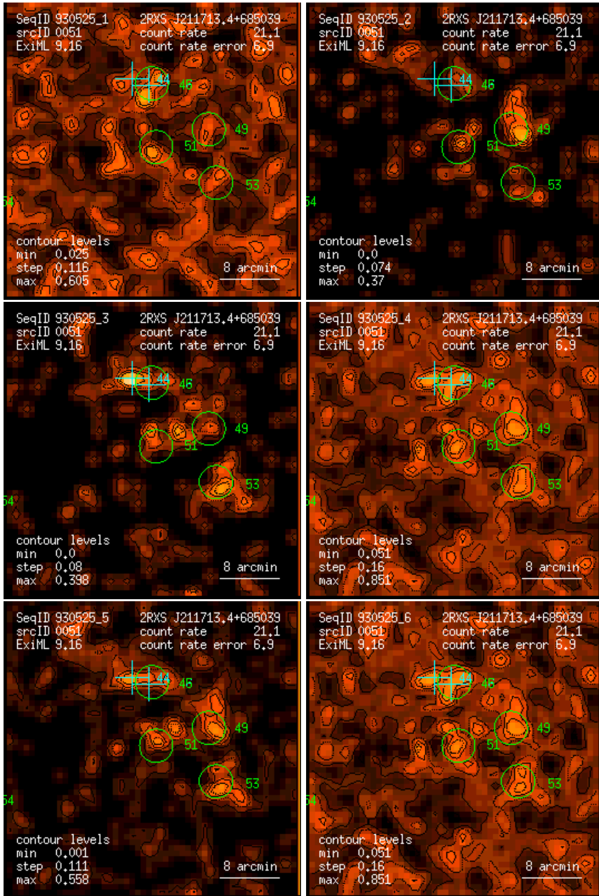
Figure 51: RASS 930525: detection 0051: band rate images, Gaussian filter: (1) PSPC channels 11 – 41, (2) 52 – 90, (3) 91 – 201, (4) 11 – 235, (5) 52 – 201, (6) 11 – 201. Broad band rates in counts/ks. Band rate contour levels in counts/ks/arcmin 2 .
